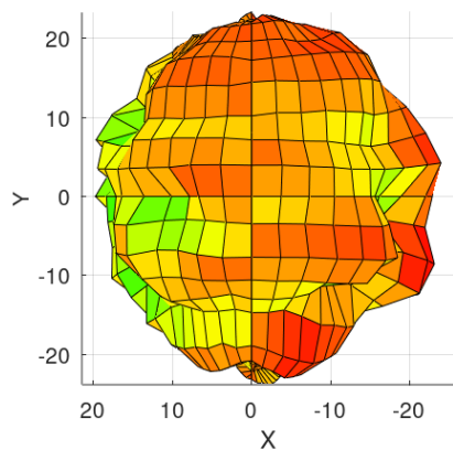
Total EIRP [dBm], Top View Azimuth = 0°, elevation = 0°
