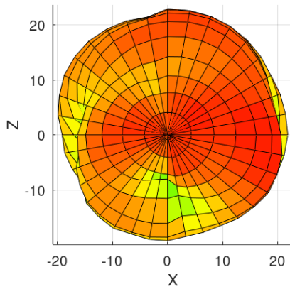
Total EIRP [dBm], Left Side View Azimuth = 0°, elevation = 90°
