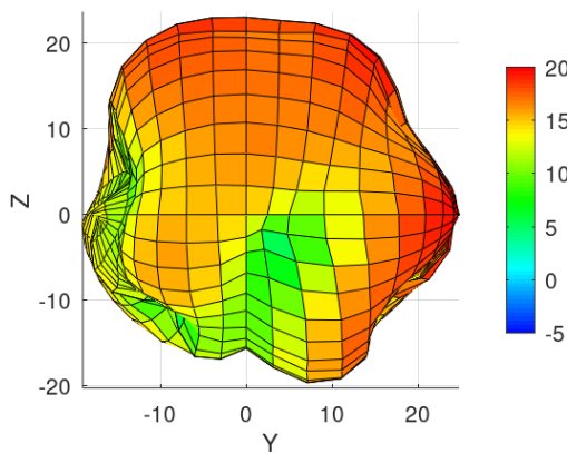
Total EIRP [dBm], Front Face View Azimuth = 90°, elevation = 0°
