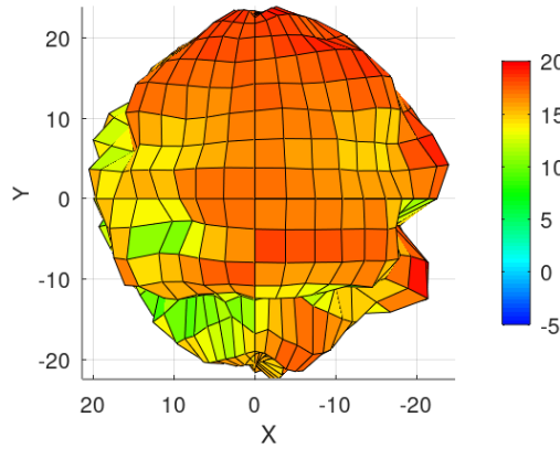
Total EIRP [dBm], Top View Azimuth = 0°, elevation = 0°
