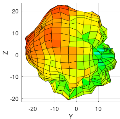
Total EIRP [dBm], Front Face View Azimuth = 90°, elevation = 0°
