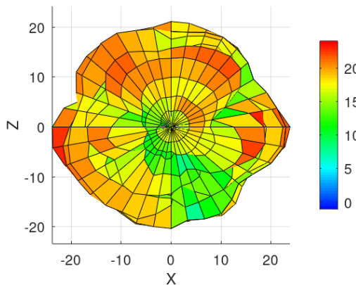
Total EIRP [dBm], Left Side View Azimuth = 0°, elevation = 90°
