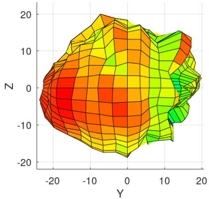
Total EIRP [dBm], Front Face View Azimuth = 90°, elevation = 0°
