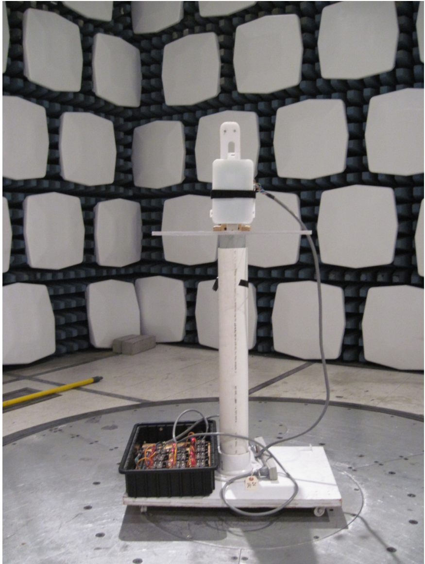
Full View of EUT during Radiated Emissions Testing
