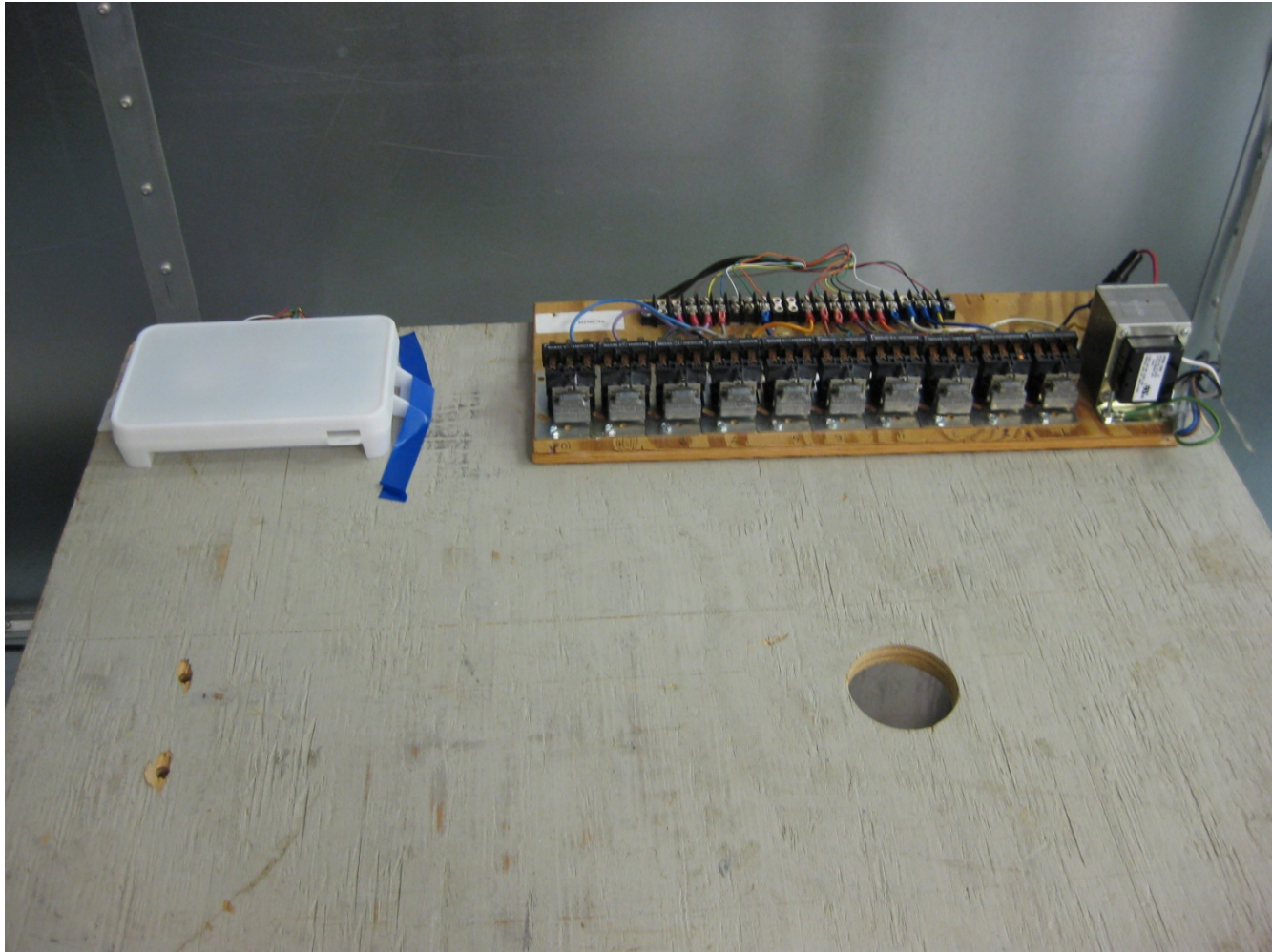
Setup for Conducted Emissions
