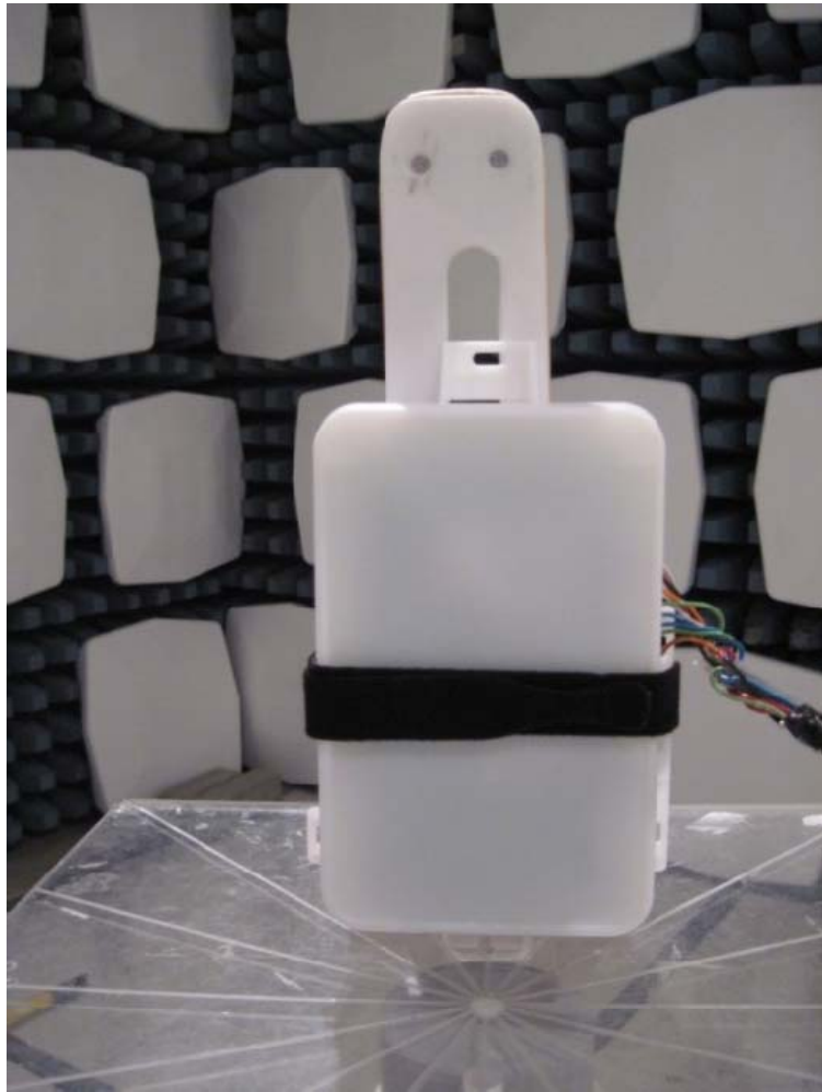
EUT on Test Pedestal for Radiated Emissions
