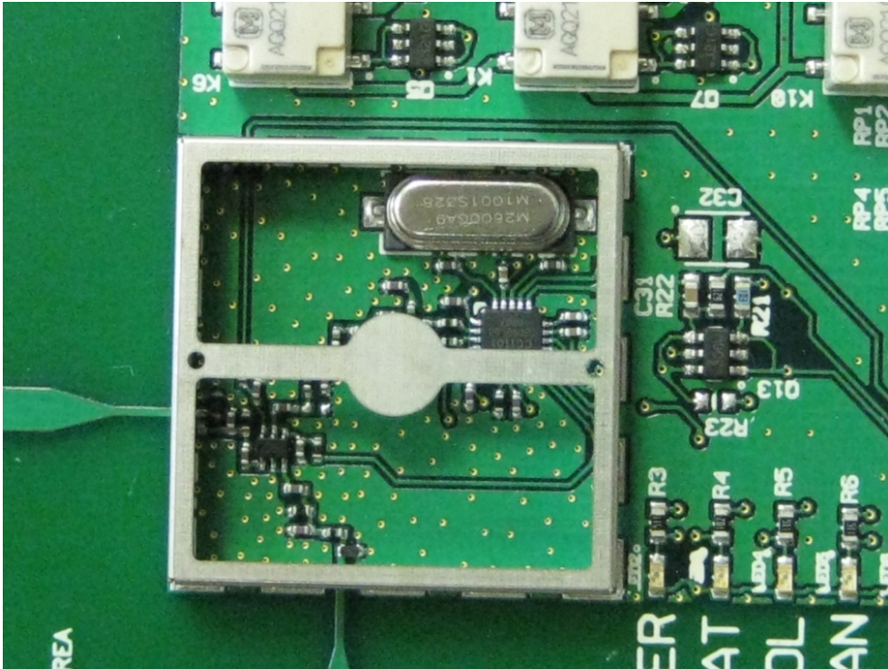
Internal Photo with Shield Removed
