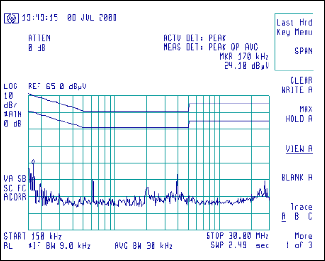
914.6 MHz, Line 1
