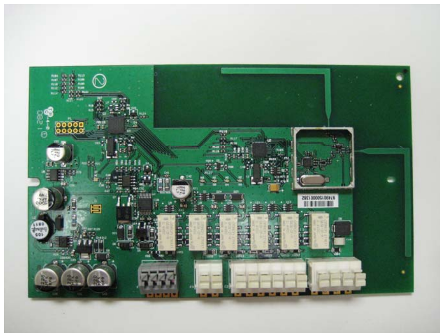
View #2 of Board
