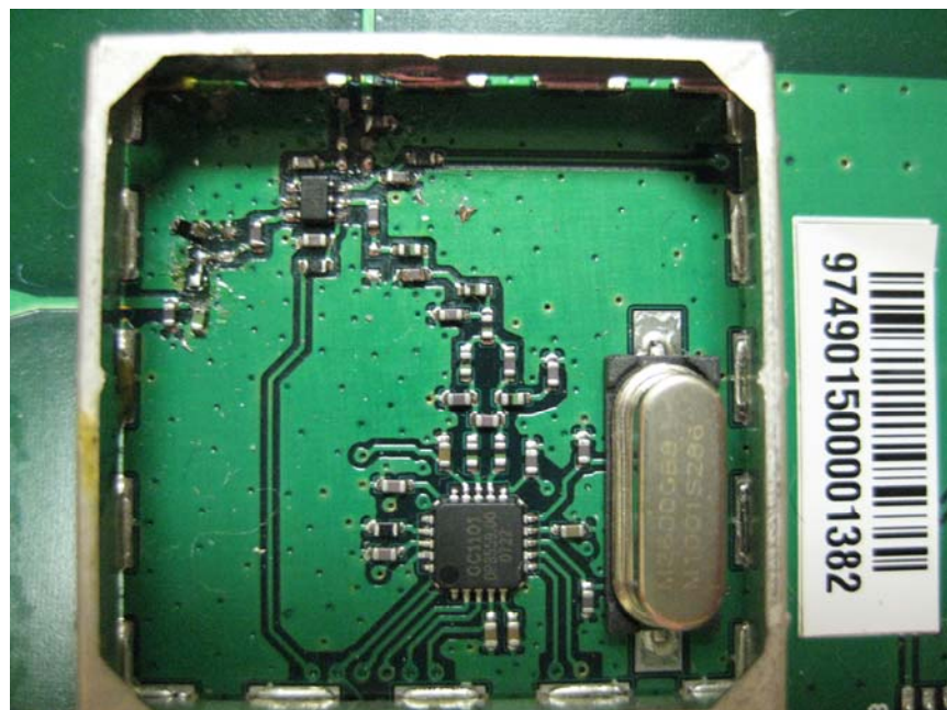
View #2 of RF Section-Unshielded
