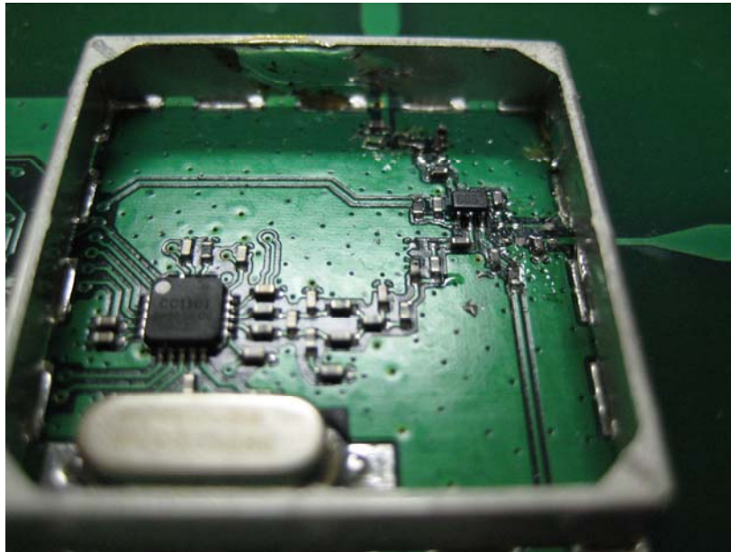
View #4 of RF Section-Unshielded
