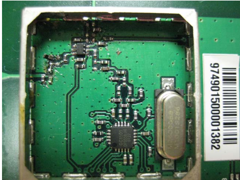
Close-Up of RF Section-Unshielded
