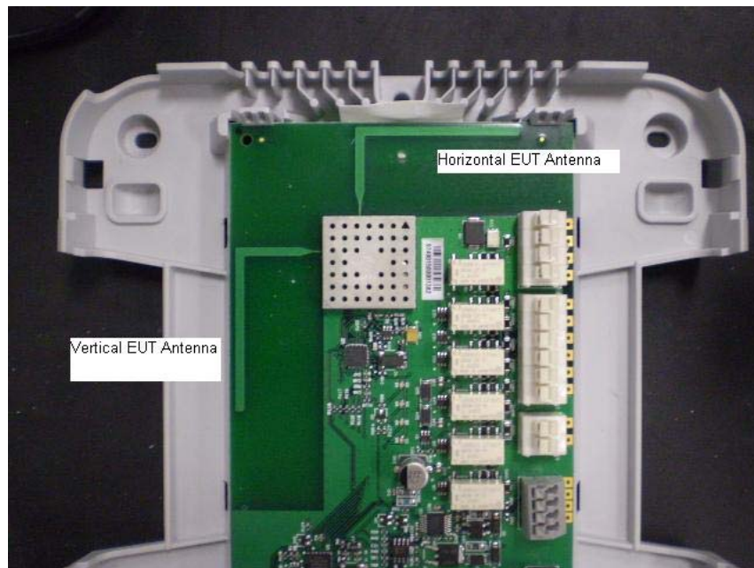
View showing placement of horizontal and vertical antennas
