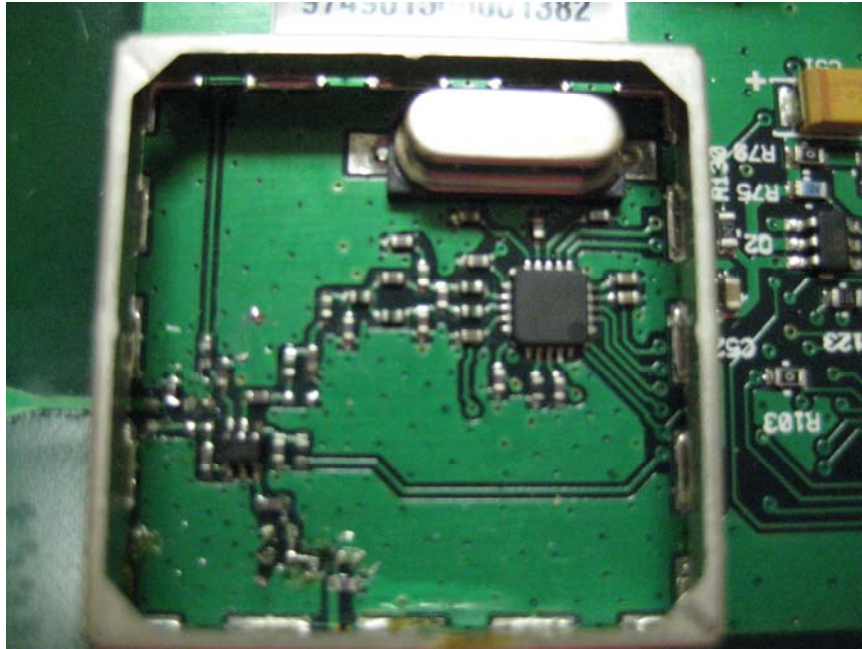
View #1 of RF Section-Unshielded
