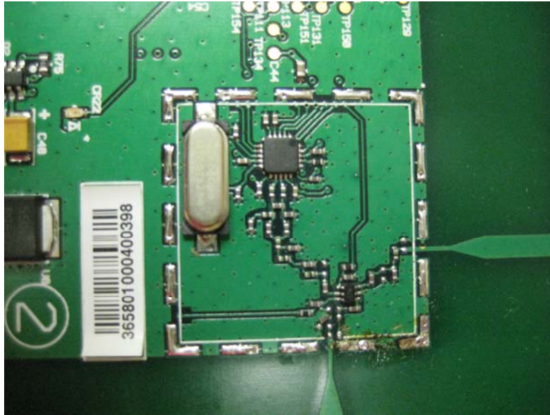
Close-Up of RF Section, Unshielded View #1
