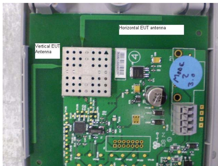
View of Vertical and Horizontal Antenna Placement
