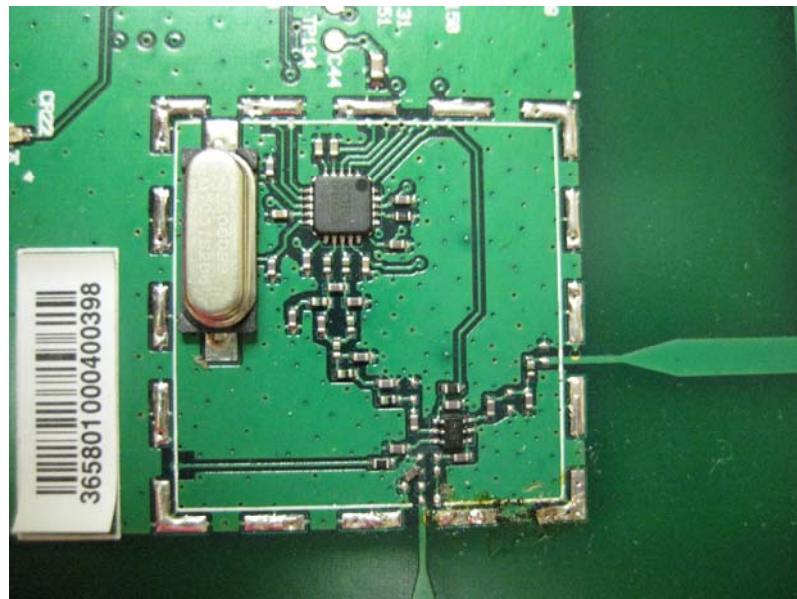
Close-Up of RF Section, Unshielded View #2
