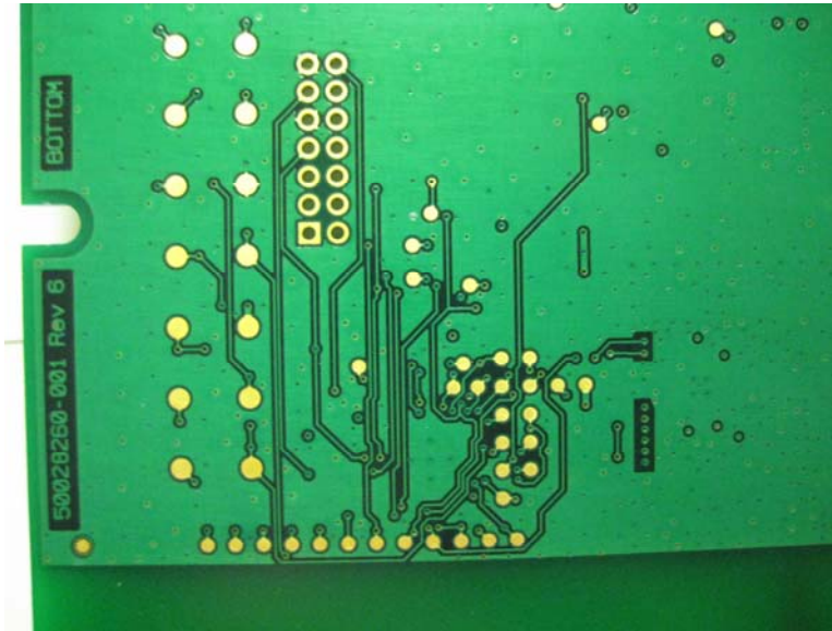
Close-Up of Back Side of Board
