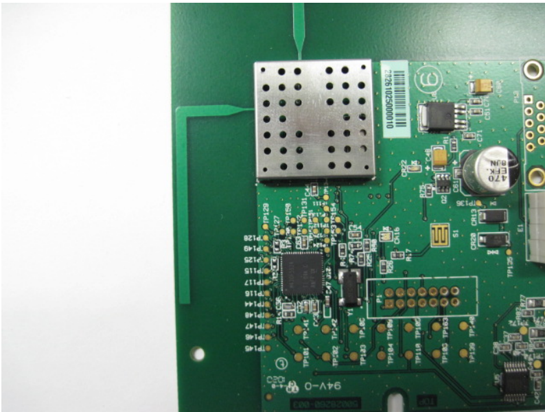
Close-up of RF Section and Antennas with Shield
