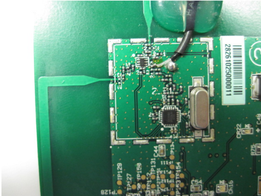
Close-up of RF Section with Shield Removed. Cable was used for Conducted measurements only. Cable is not present in final product.
