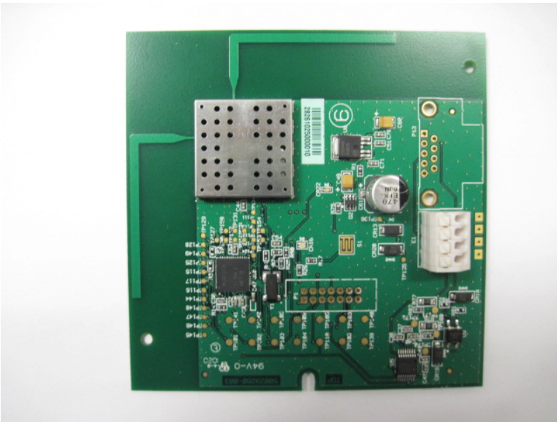
Close-up of Front Side of RF Board
