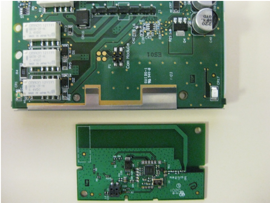
Boards separated with enclosure removed
