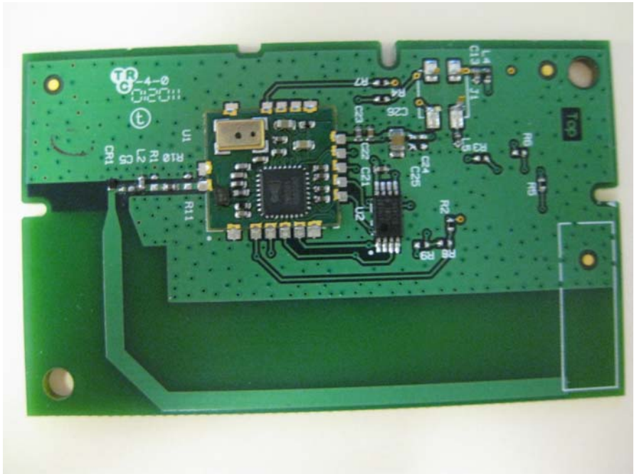
Close up of top side on radio board and PCB antenna
