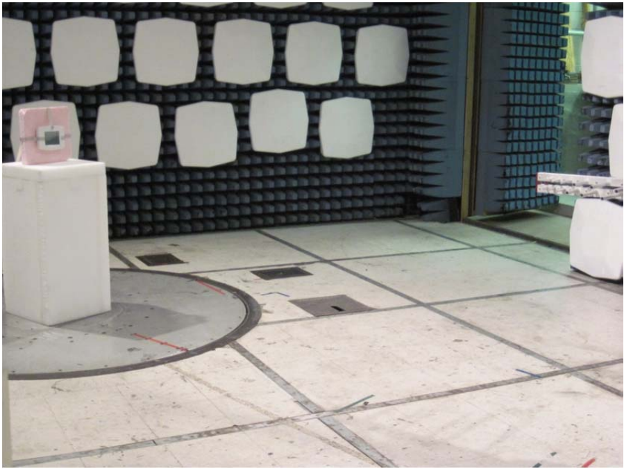
Demonstrates EUT & receive antenna relative placement
