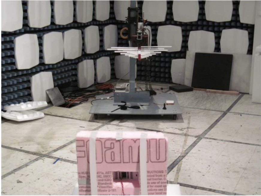
View from EUT to Receive antenna
