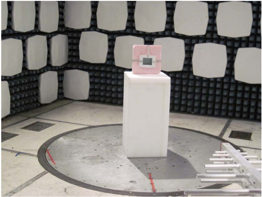
View from receive antenna to EUT
