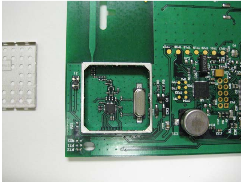
RF Section – Shield Removed
