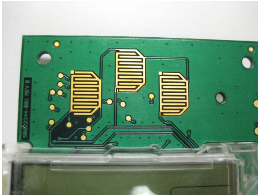
Close Up View #2 of Portion of Back Side of Board
