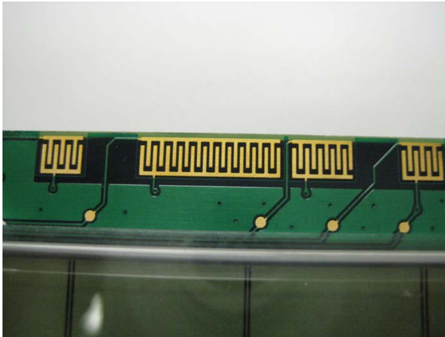
Close Up View #1 of Portion of Back Side of Board
