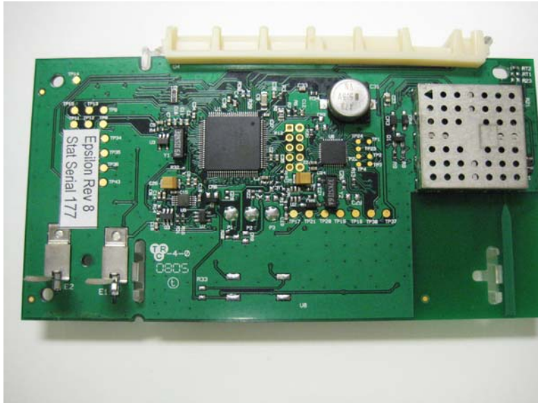
Board - RF Section Shielded View #1
