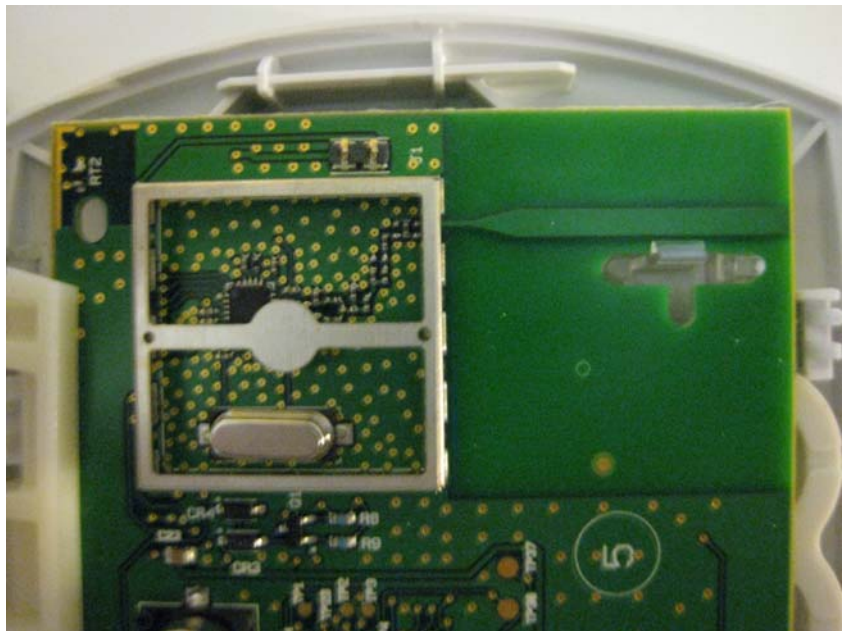
Close-up of trace antenna
