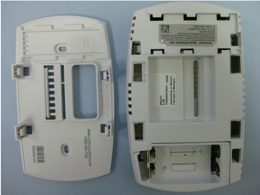
Unit with back plate removed
