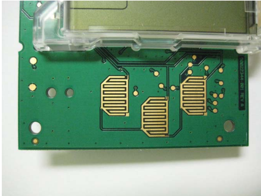
Close Up View #1 of Portion of Back Side of RF Board
