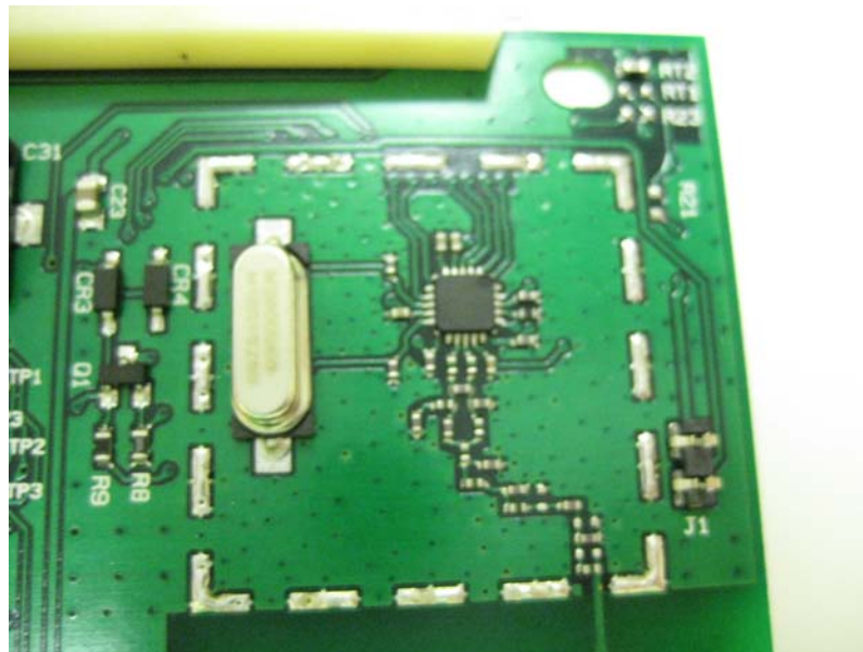
Close Up View #1 of RF Section
