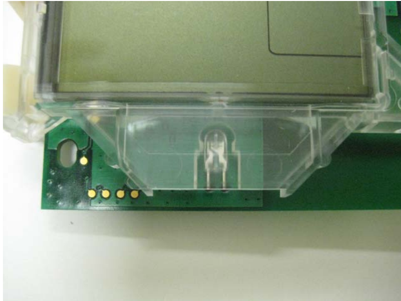
Close Up View #3 of Portion of Back Side of RF Board
