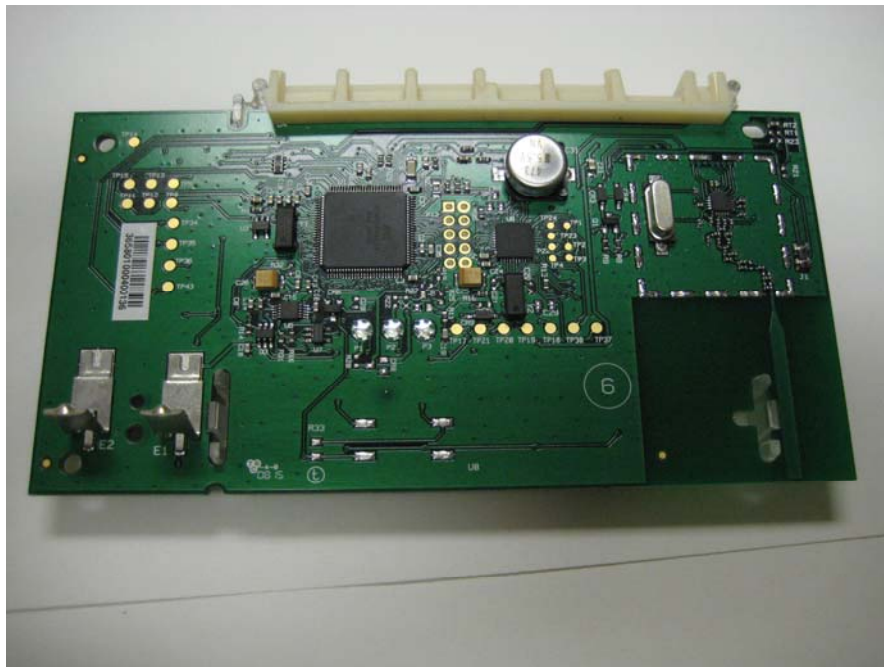
View #3 of RF Section
