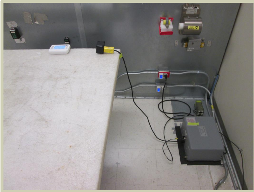
Powerline Conducted Emissions
