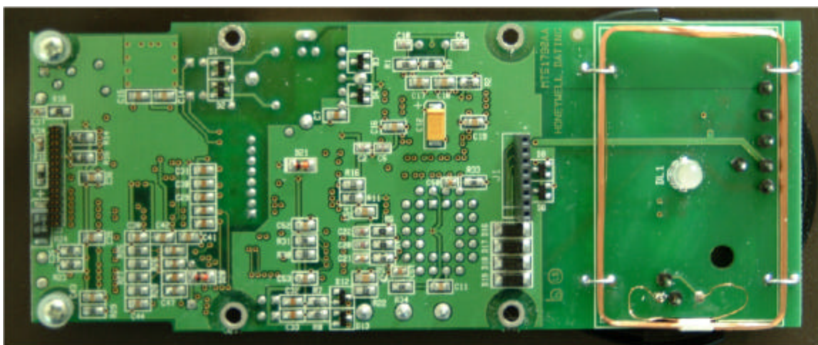
FIG8-7 CPU board Side 2
