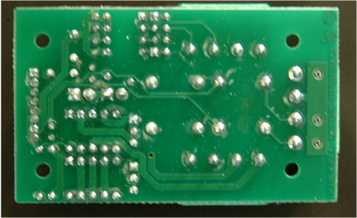
FIG8-5 I/O card side 2
