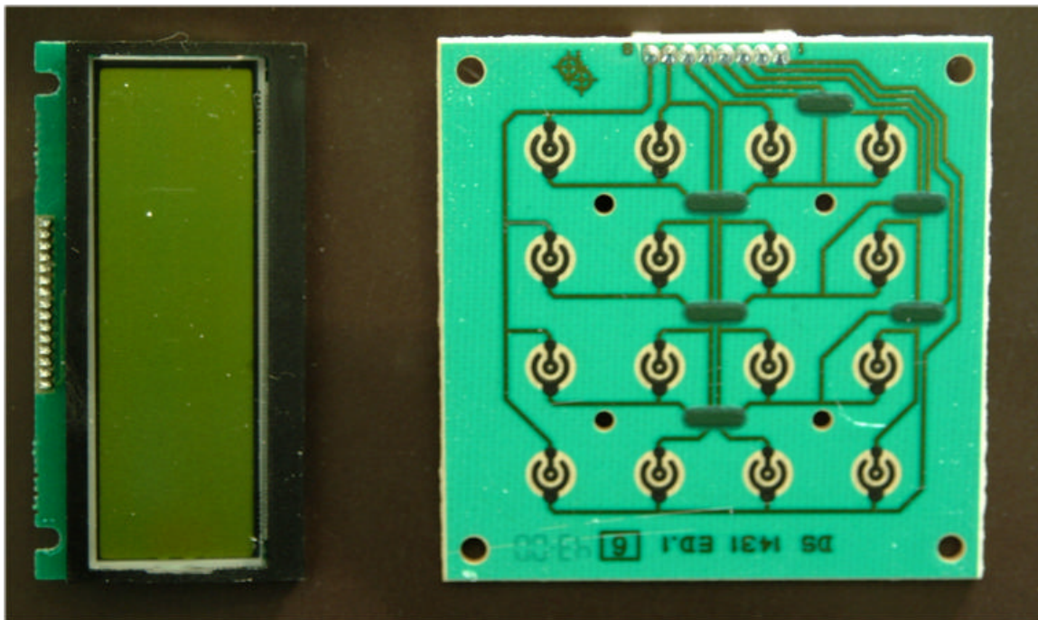
FIG8-10 Keyboard and display units side 1
