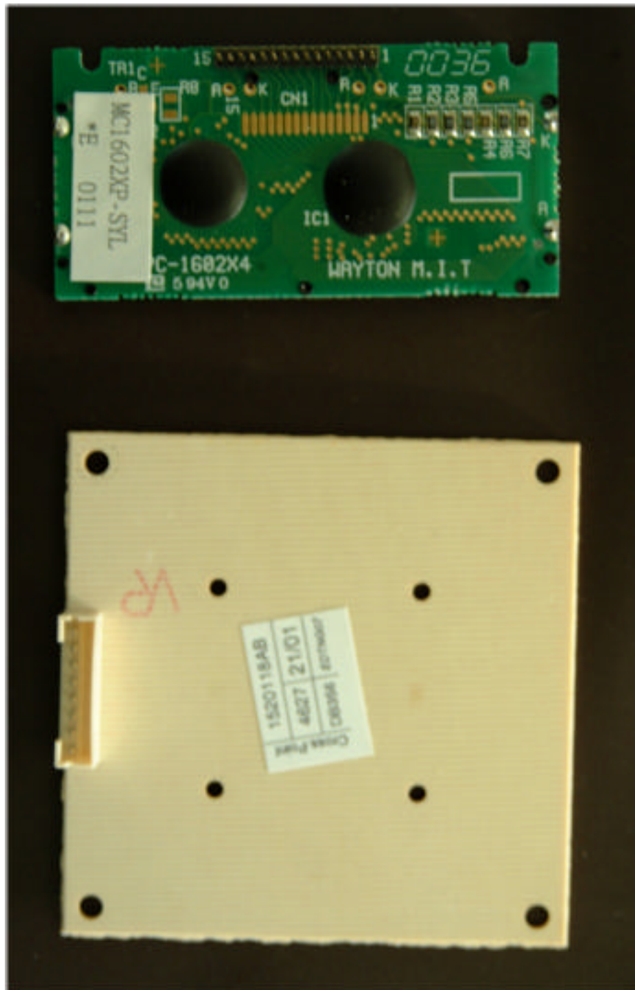
FIG8-11 Keyboard and display units side 2
