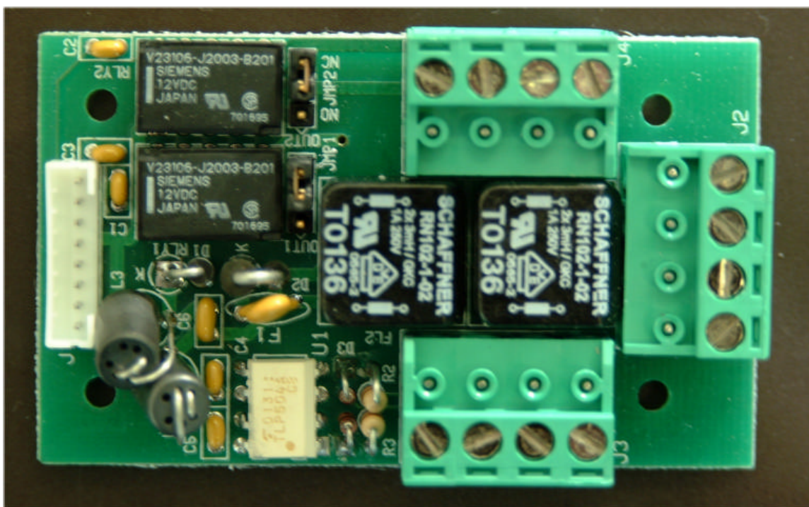
FIG8-4 I/O card side 1
