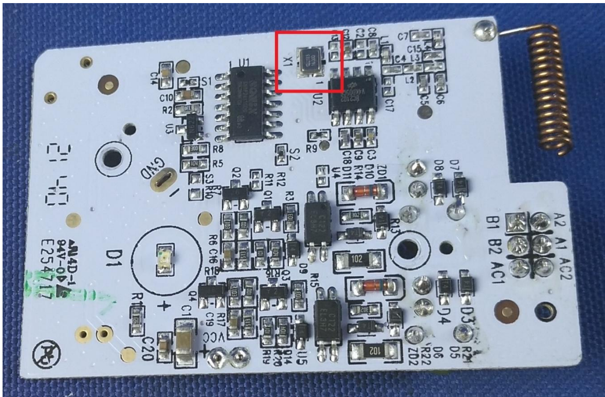
Oscillator Location
