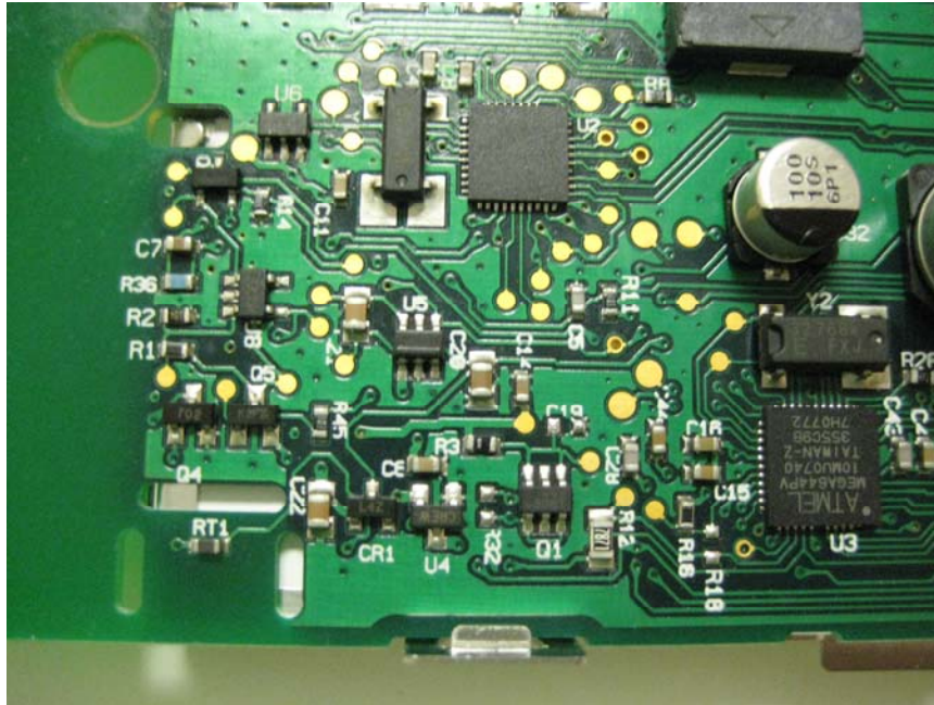
Close-Up of RF Section View #1
