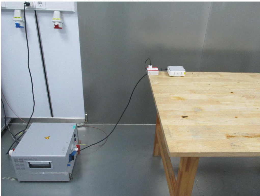
Conducted emission at AC mains
