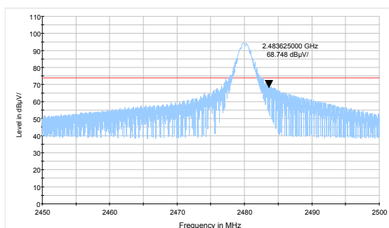
3DH5-Channel 78: Peak
