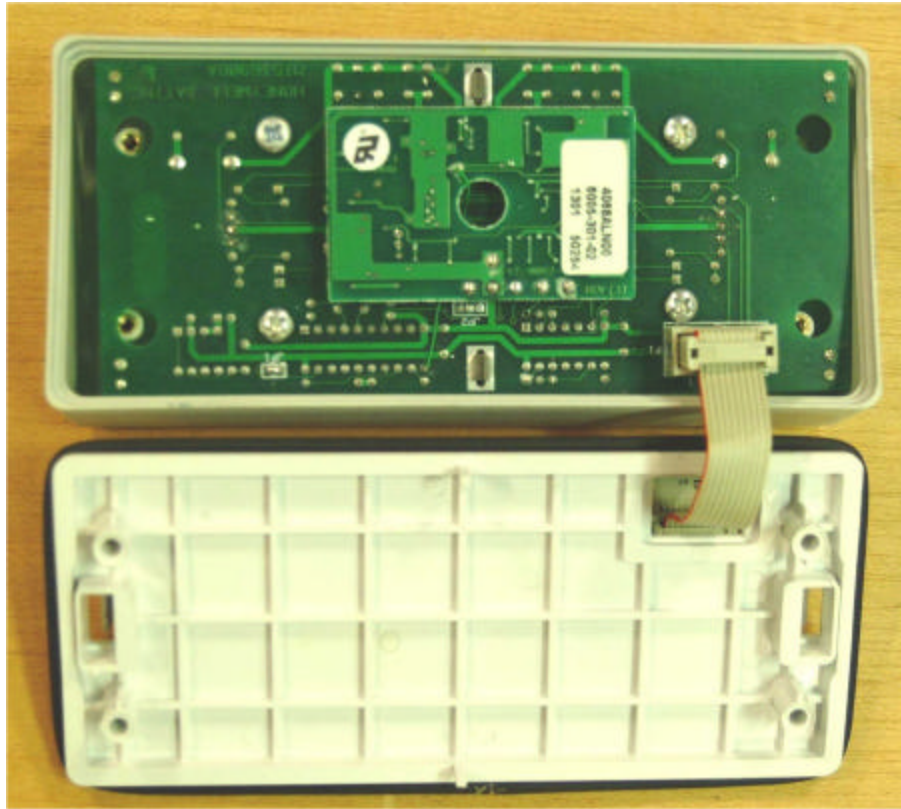
UNIT PARTIALLY DISASSEMBLED
