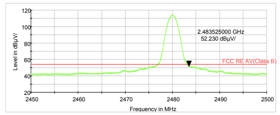
Zigbee-Channel 26: Average
