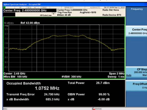
BLE V5.0-1M Carrier frequency (MHz): 2480
