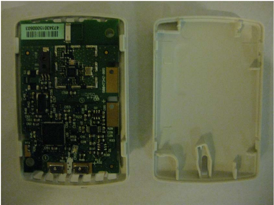
Front side of unit open for inspection
