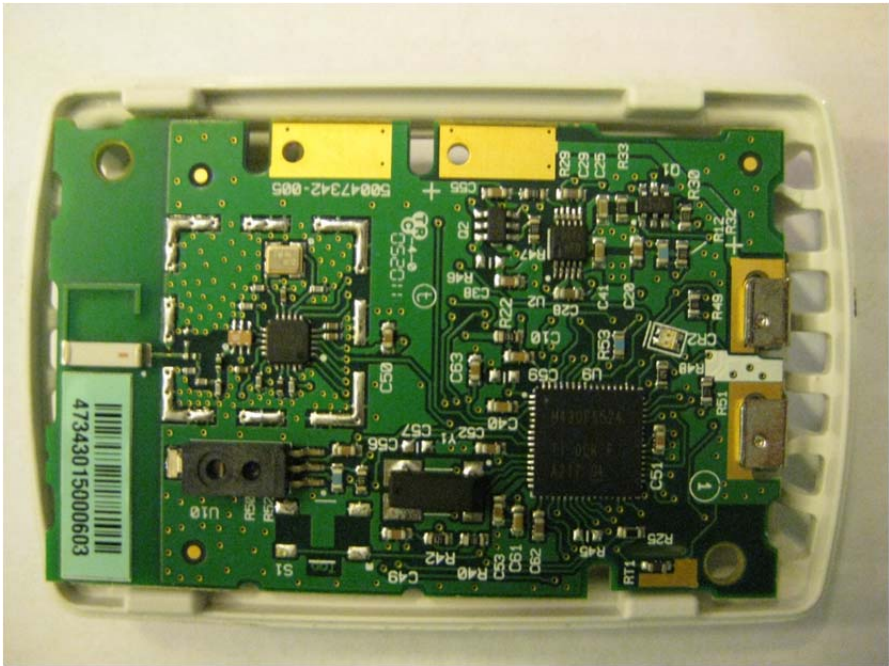
Close up of front side of board
