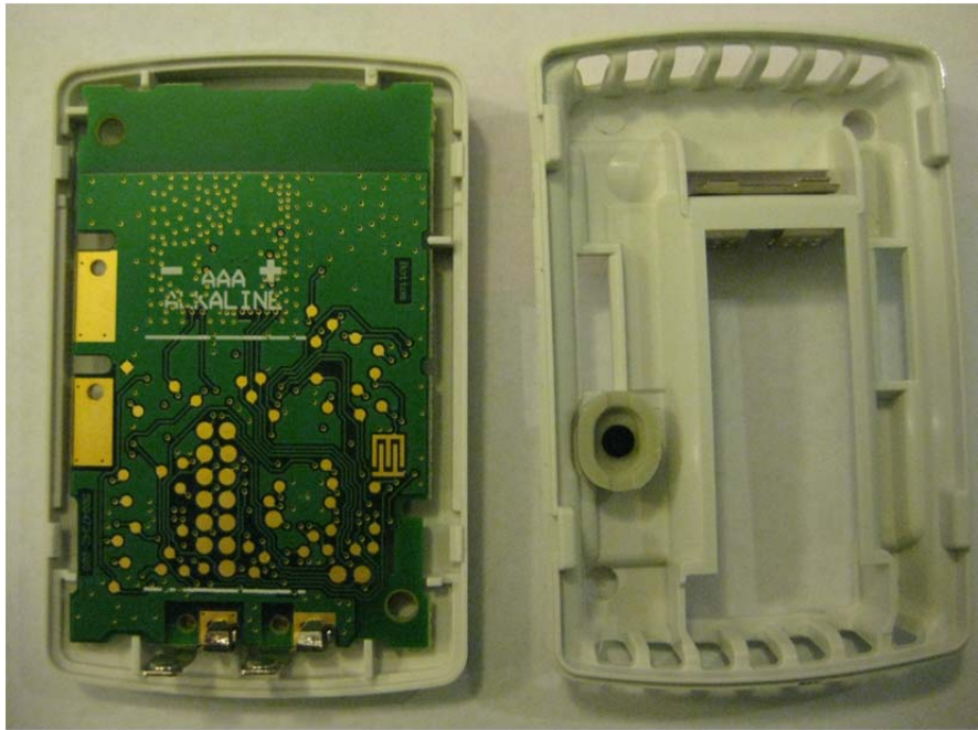
Back side of unit open for inspection
