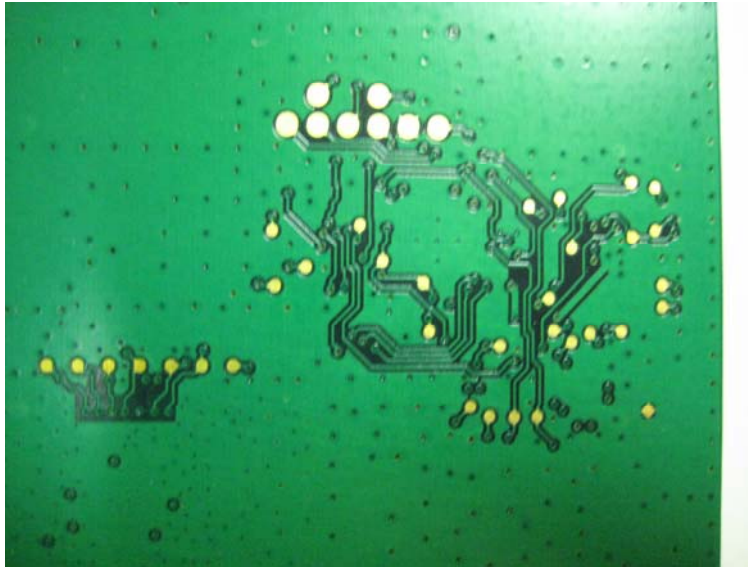
View #3 – Back Side of Board – Close Up
