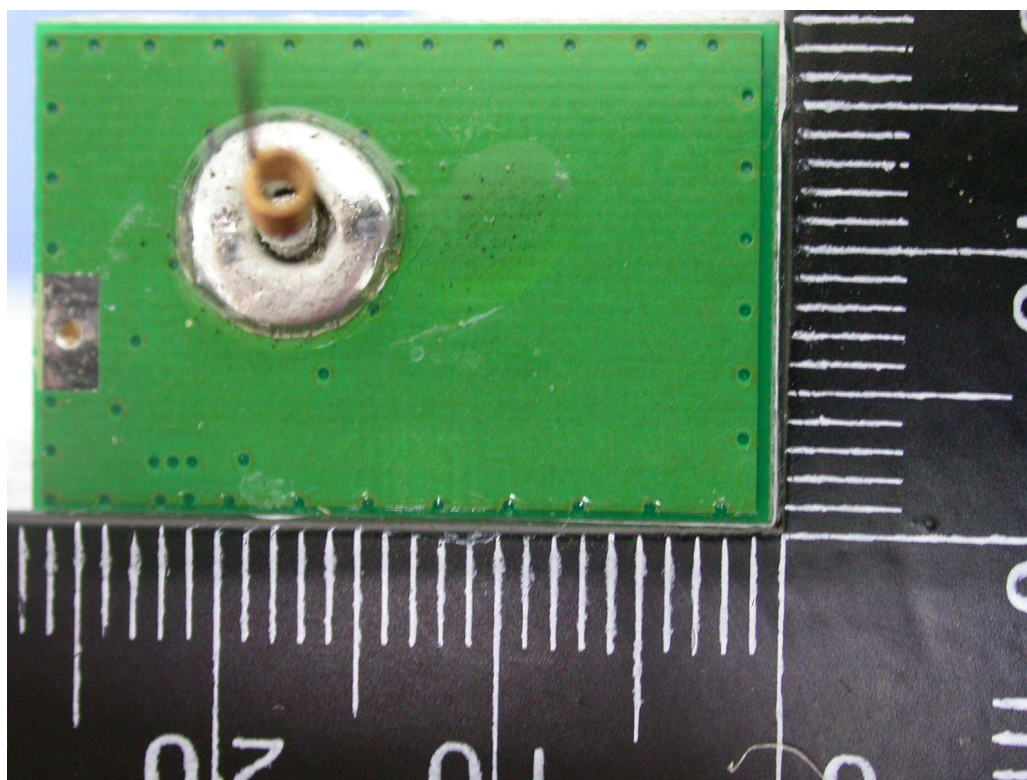
14. Rear view of PCB3
