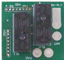
RLY Transmit/Receive Relay Board Component Side
