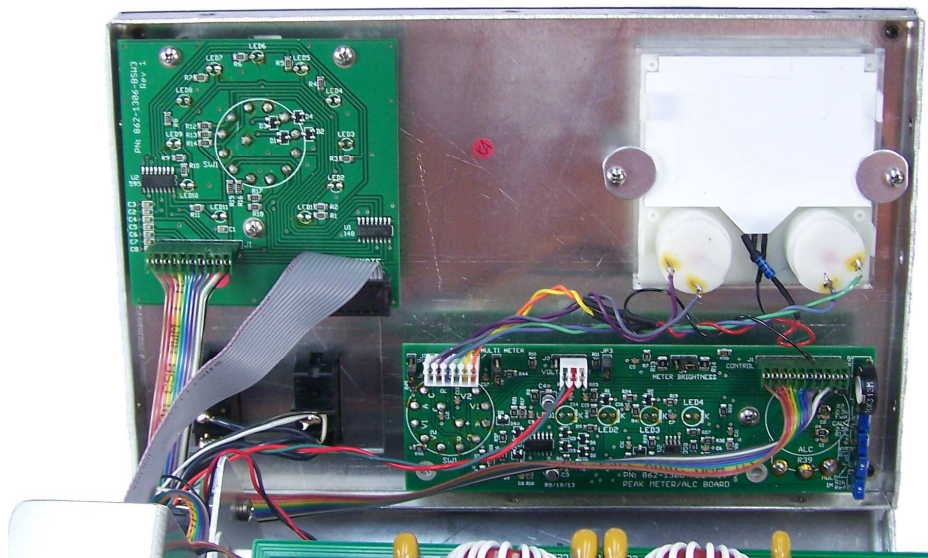
ALS-706 Front Panel with BSW3 Board and MB2 Meter Board
