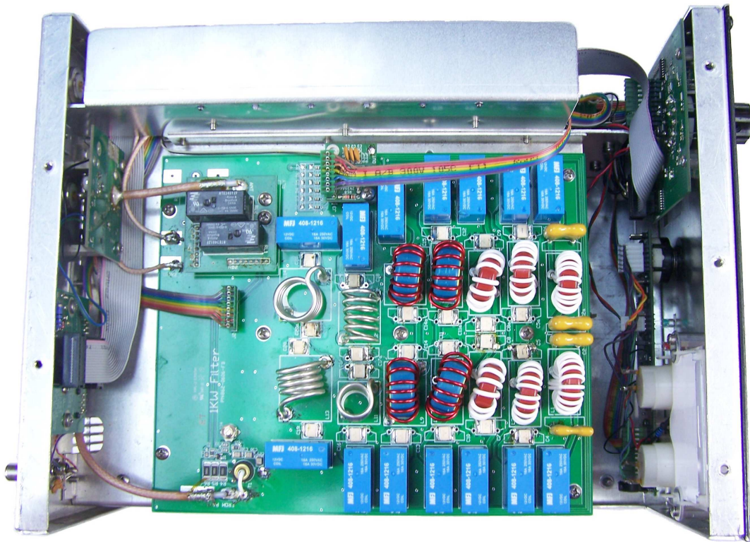
ALS-706 Top View with 1KWF6 Board
