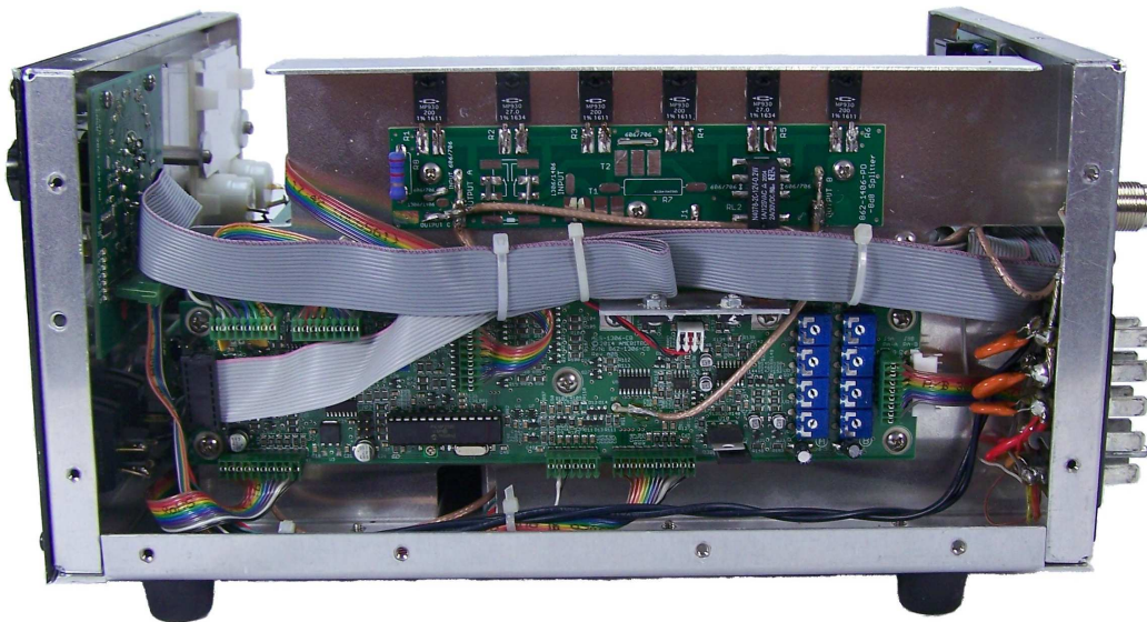
ALS-706 Right Side View with CB2 Control Board and PD8M wired for ALS-706.
