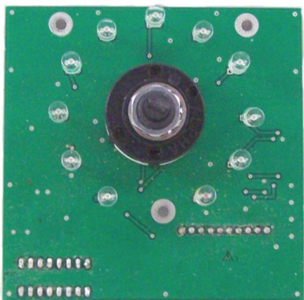
BSW3 Band Switch Board Bottom Side
