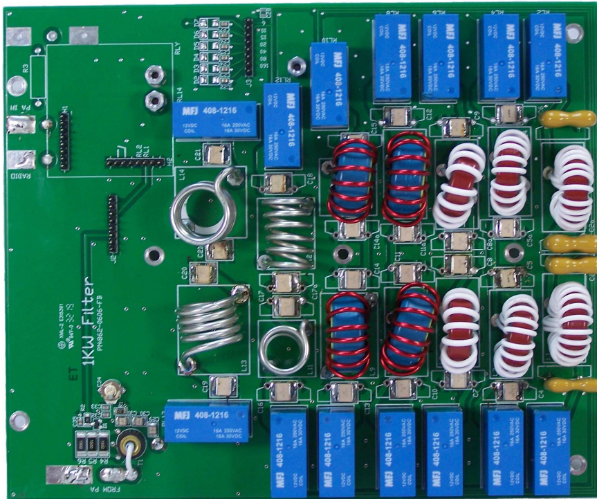
1KWF6 Filter Board Component Side
