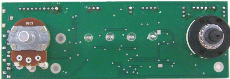
MB2 Meter Board Bottom Side
