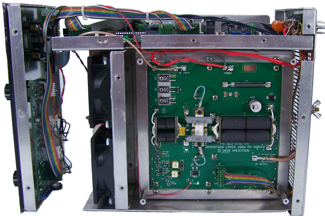
ALS-706 Bottom View with PAM-706 Module
