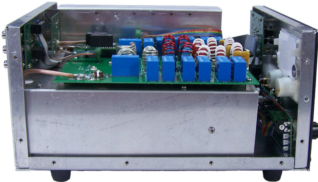
ALS706 Left Side View
