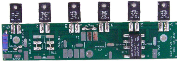
PD8M Attenuator Board Component Side wired for ALS-706
