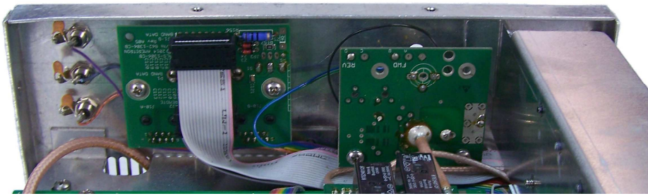
ALS-706 Rear Panel with RJ45 Board and SWR Board
