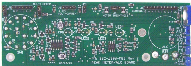
MB2 Meter Board Component Side
