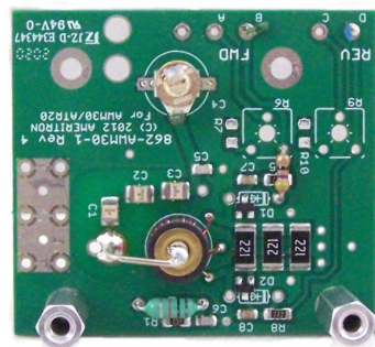
SWR Board Component Side
