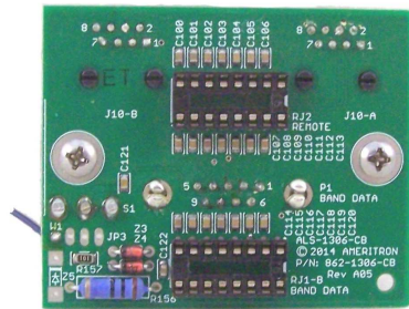
RJ45 Radio Interface Board Component Side
