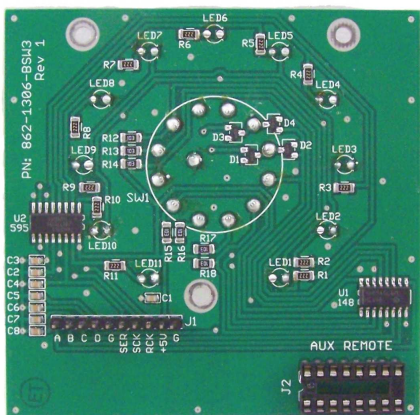
BSW3 Band Switch Board Component Side
