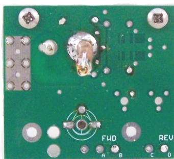
SWR Board Bottom Side
