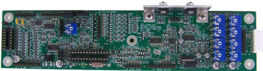
CB2 Control Board Component Side
