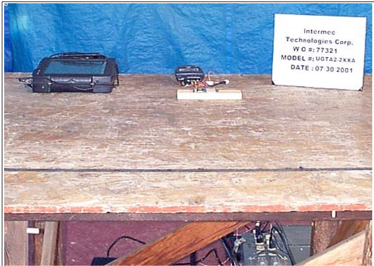
Radiated Emissions - Orthogonal A Front View
