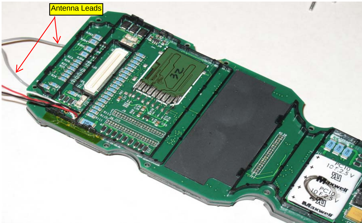
Top Board – Display removed
