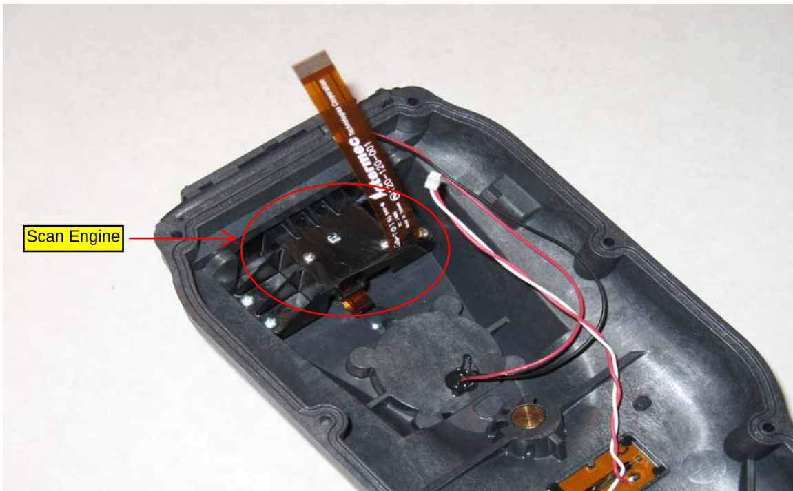
Bottom Enclosure Removed
