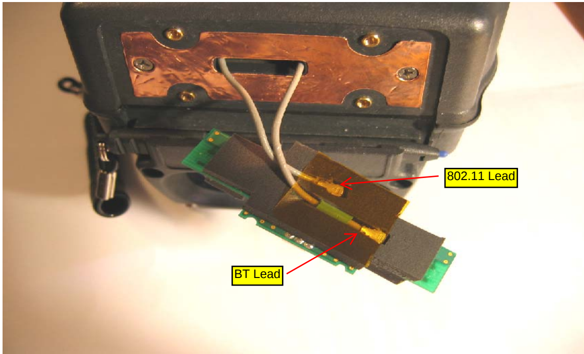
Antenna Lead Connections
