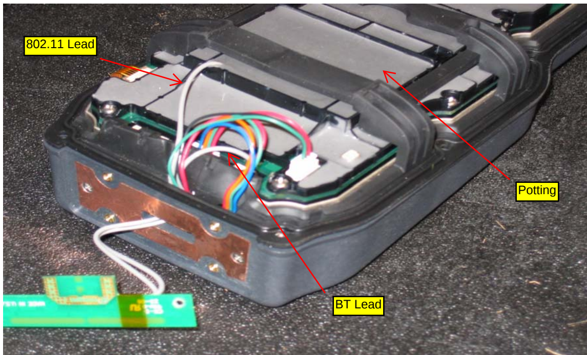
Bottom Enclosure Removed – Potting
