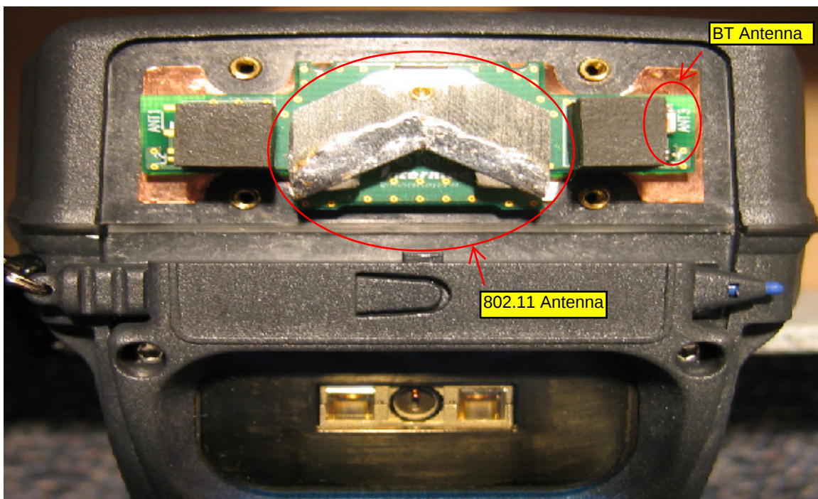
Antenna Board – WiFi and BT Antennas
