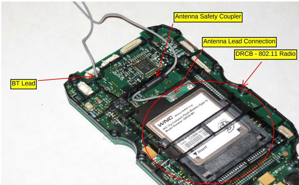
DRCB Radio – Bottom Board
