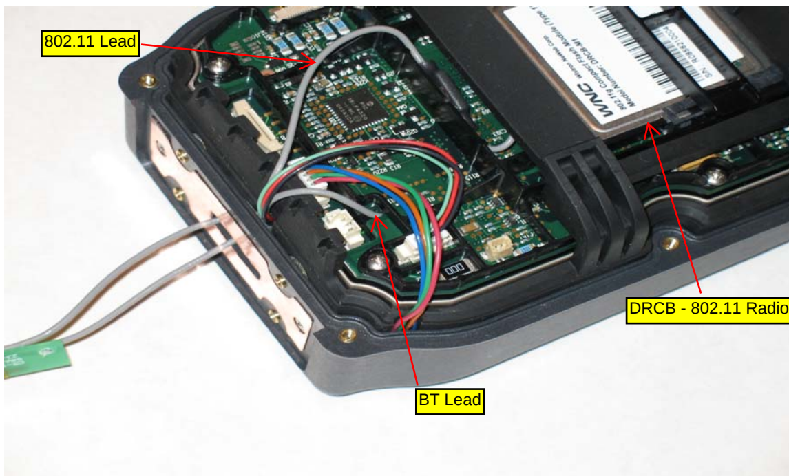
Bottom Enclosure Removed – No Potting: DRCB Radio
