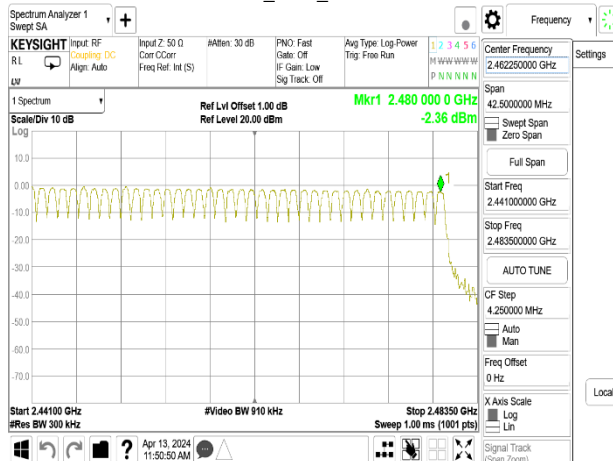
GFSK_2.4G_2441-2480
