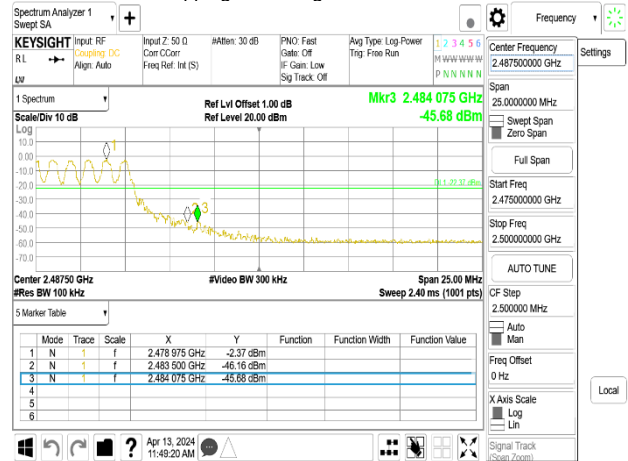
Hopping Band Edge_2.4G_2480MHz
