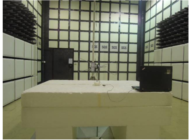
FCC 15 247 2.4G Radiated Setup
