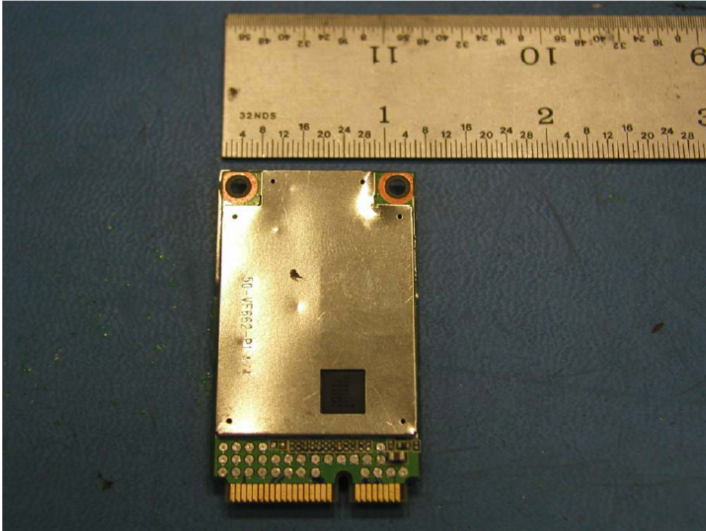
Figure 1 JTAG side
