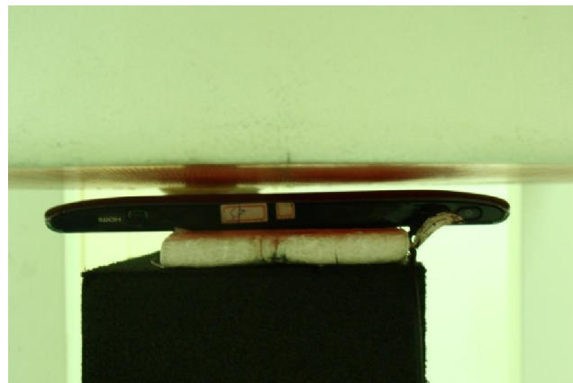
Rear Face of the DUT with Phantom 5 mm Gap (Voluntarily submitted)
