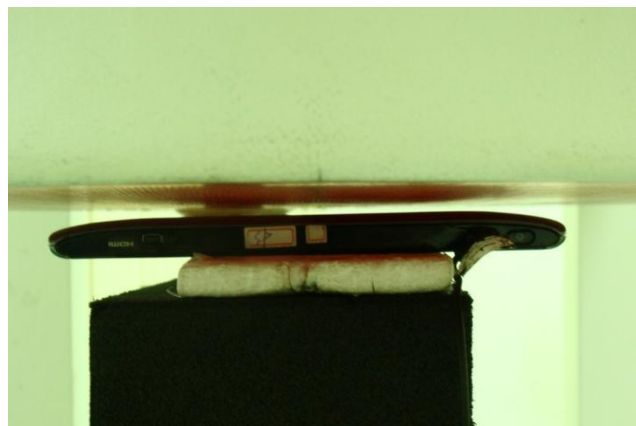
Rear Face of the DUT with Phantom 5 mm Gap
