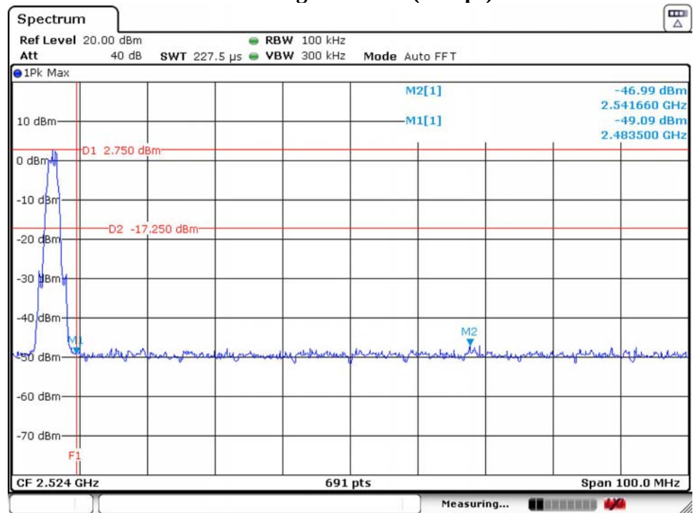
GFSK High Channel (2Mbps)
