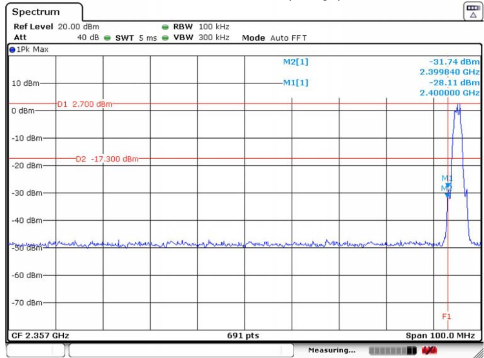
GFSK Low Channel (2Mbps)
