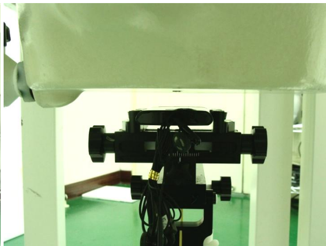
Bottom of the DUT with Phantom 1.5 cm Gap with Earphone 2 for Sample A
