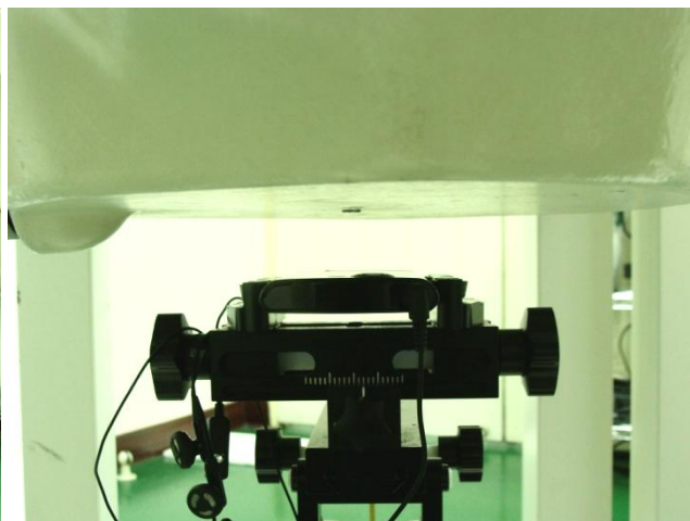
Bottom of the DUT with Phantom 1.5 cm Gap with Earphone 1 for Sample A
