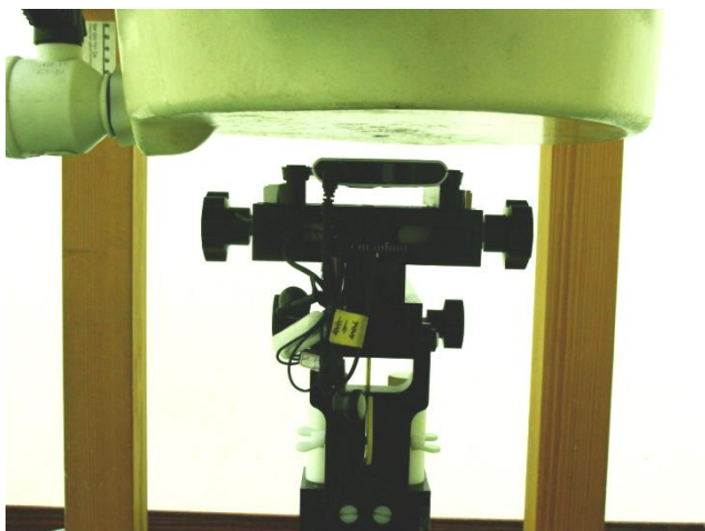
Face of the DUT with Phantom 1.5 cm Gap (With Earphone 1)
