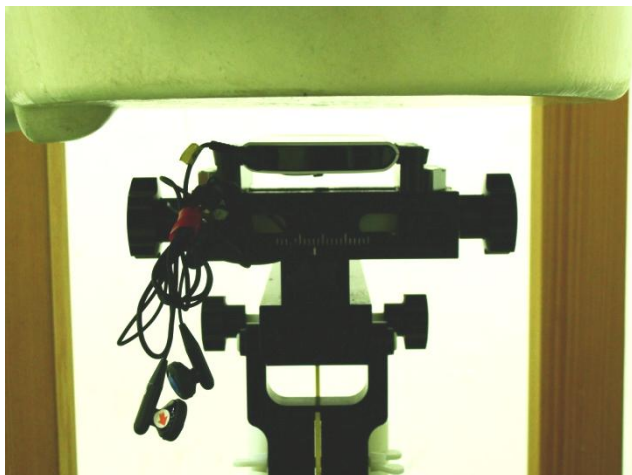
Face of the DUT with Phantom 1.5 cm Gap (With Earphone 2)
