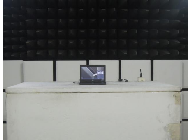
FCC_96_LTE_Radiated_Setup
