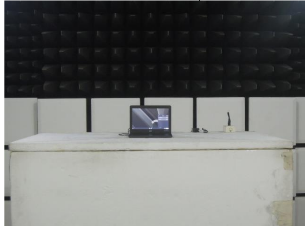
2_3G_Radiated_Setup
