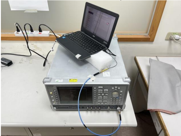
LTE_Conducted_Setup
