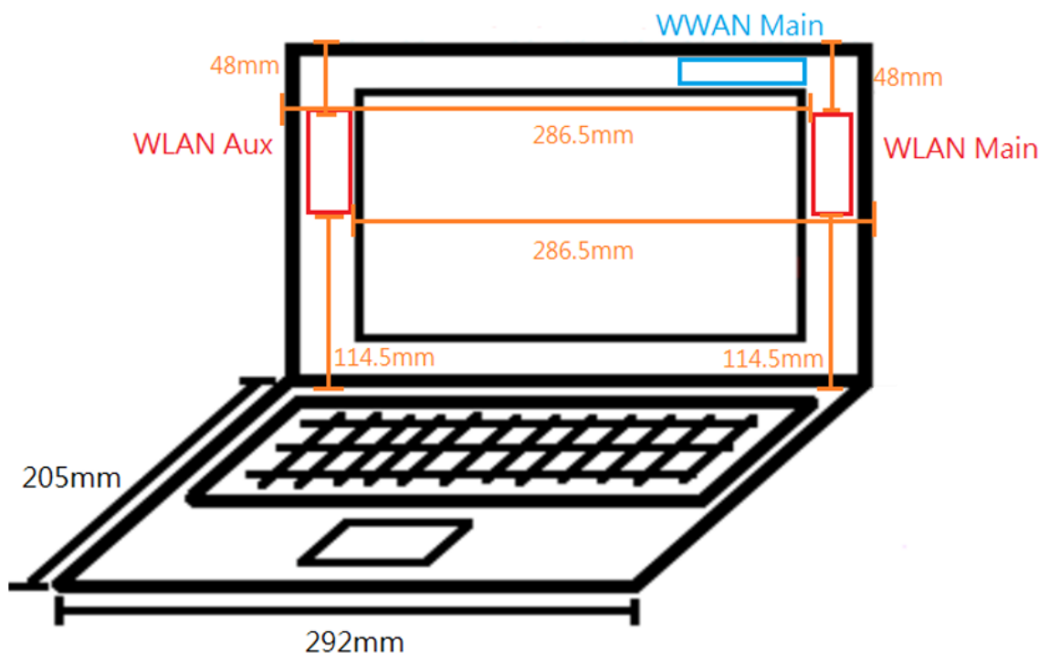
Photograph 5. Antenna position of EUT
