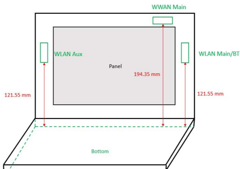
Fig.6 Antenna location of EUT
