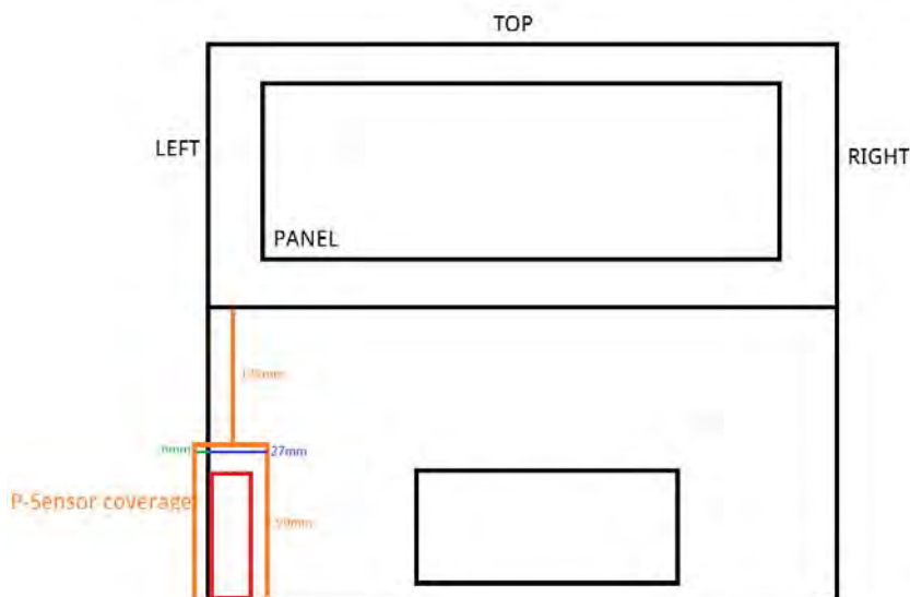
Fig.7 Antenna position of EUT
