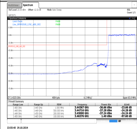
Band42(3450-3550)-15MHz-QPSK-43015-1RB#0-PASS
