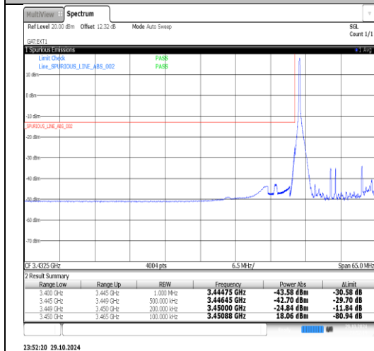
Band2(3450-3550)-15MHz-16QAM-42165-1RB#74-PASS
