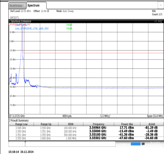
Band42(3450-3550)-5MHz-16QAM-42115-25RB#0-PASS
