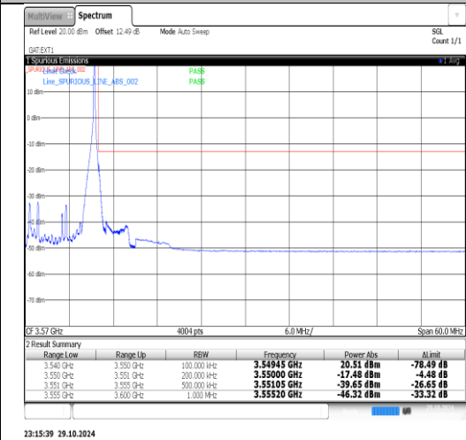
Band2(3450-3550)-10MHz-16QAM-42140-50RB#0-PASS
