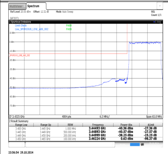
Band2(3450-3550)-15MHz-16QAM-43015-1RB#0-PASS
