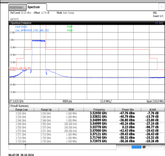
42(3550-3600)-20MHz-16QAM-43490-1RB#0- PASS
