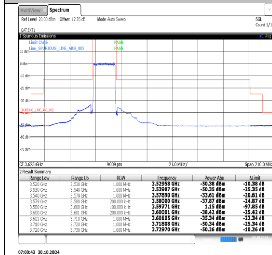
42(3550-3600)-20MHz-16QAM-43190-1RB#0- PASS
