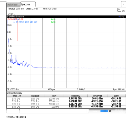
Band42(3450-3550)-5MHz-QPSK-43065-1RB#24-PASS
