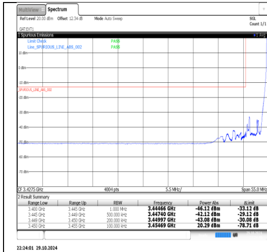
Band42(3450-3550)-5MHz-QPSK-43065-25RB#0-PASS
