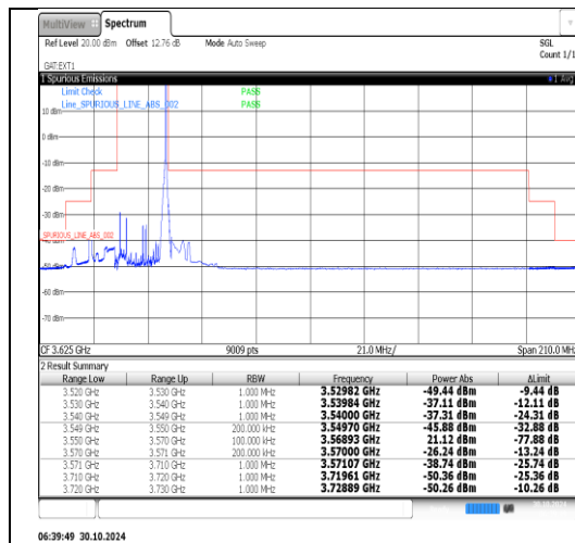
42(3550-3600)-20MHz-QPSK-43490-100RB#0- PASS
