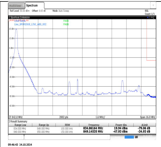
Band26(824-849)-15MHz-16QAM-26965-1RB#74-PASS
