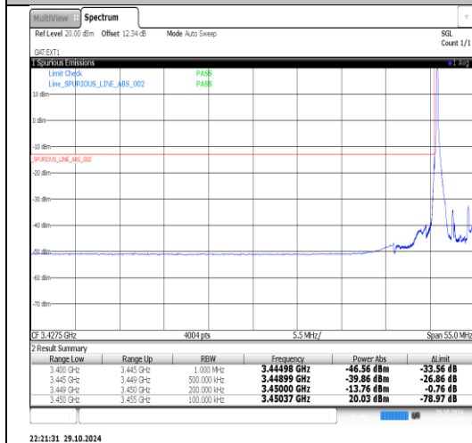
Band42(3450-3550)-5MHz-QPSK-42115-1RB#24-PASS
