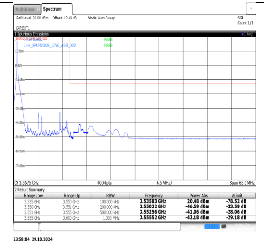
Band2(3450-3550)-15MHz-QPSK-43015-1RB#74-PASS
