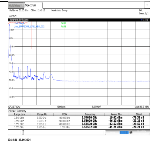
Band42(3450-3550)-10MHz-16QAM-43040-1RB#49-PASS
