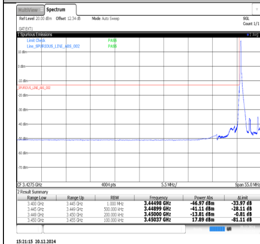
Band42(3450-3550)-5MHz-16QAM-42115-1RB#24-PASS
