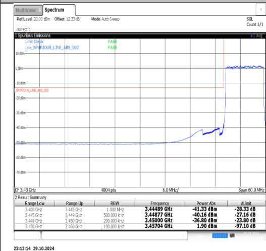
Band2(3450-3550)-10MHz-16QAM-43040-1RB#0-PASS
