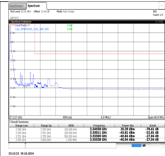
Band2(3450-3550)-10MHz-QPSK-43040-1RB#49-PASS
