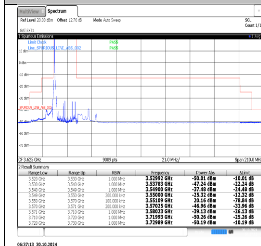
42(3550-3600)-20MHz-16QAM-43190-1RB#99- PASS
