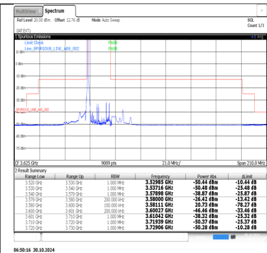
42(3550-3600)-20MHz-QPSK-43490-1RB#99- PASS
