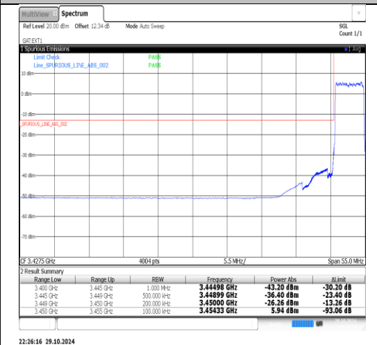
Band42(3450-3550)-5MHz-QPSK-43065-1RB#0-PASS
