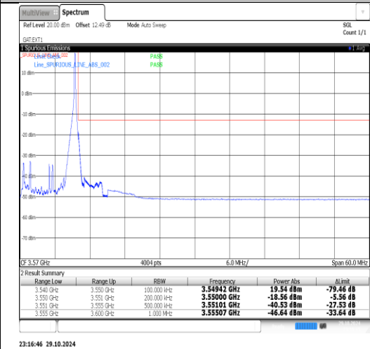
Band42(3450-3550)-15MHz-QPSK-42165-75RB#0-PASS
