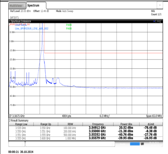
Band2(3450-3550)-15MHz-16QAM-42165-75RB#0-PASS
