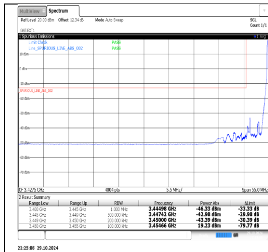
Band2(3450-3550)-5MHz-16QAM-43065-25RB#0-PASS
