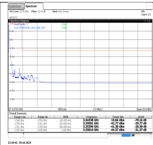
Band2(3450-3550)-5MHz-16QAM-43065-1RB#24-PASS
