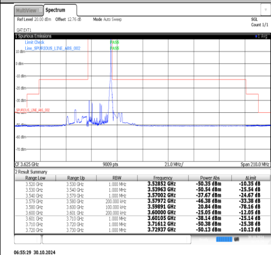
42(3550-3600)-20MHz-16QAM-43190-100RB#0 PASS
