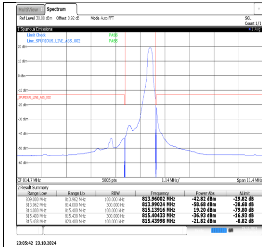
Band26(814-824)-1.4MHz-QPSK-26783-6RB#0-PASS
