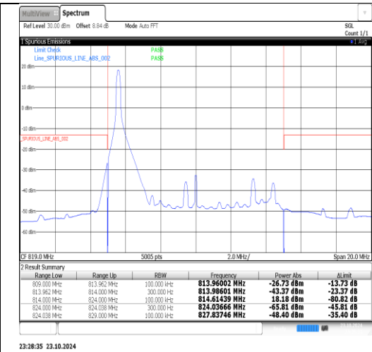
Band26(814-824)-10MHz-16QAM-26740-1RB#49-PASS
