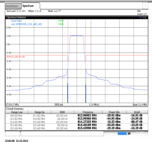
Band26(814-824)-1.4MHz-QPSK-26783-1RB#0-PASS
