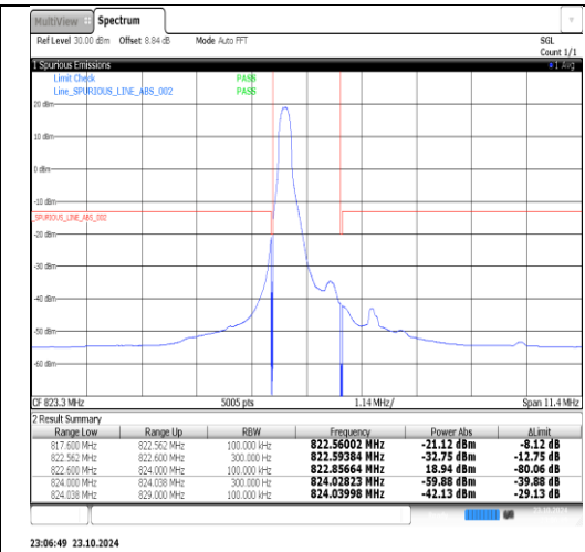
Band26(814-824)-1.4MHz-16QAM-26783-1RB#5-PASS
