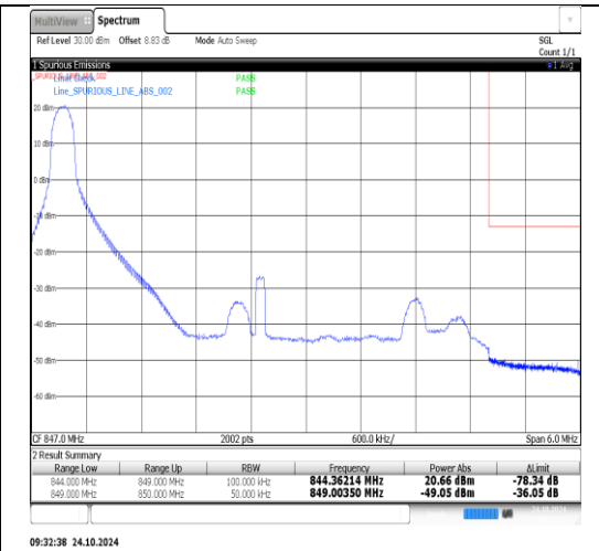
Band26(824-849)-5MHz-16QAM-27015-1RB#24-PASS
