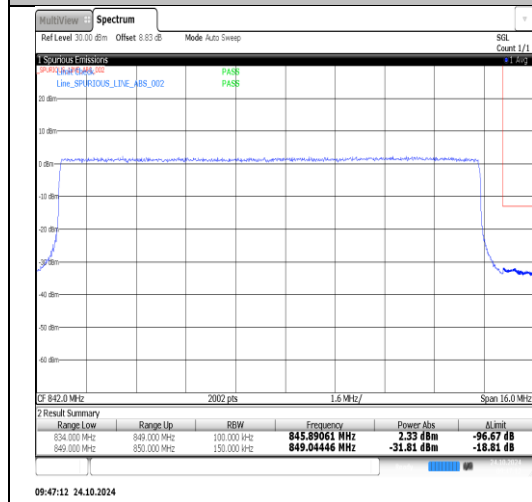
Band26(824-849)-15MHz-16QAM-26865-1RB#0-PASS
