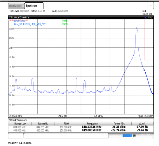
Band26(824-849)-15MHz-16QAM-26865-75RB#0-PASS
