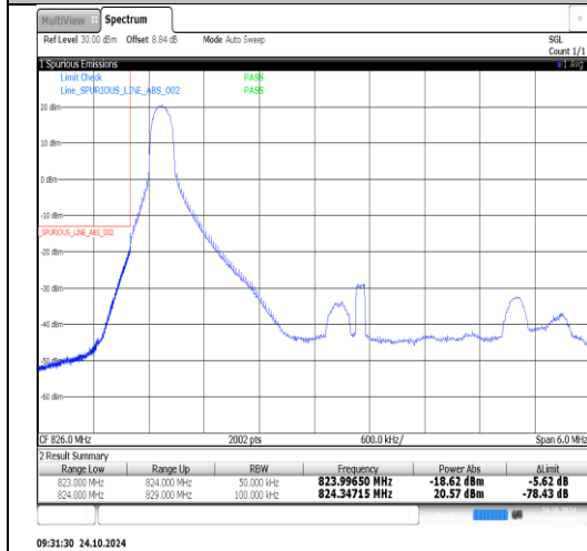
Band26(824-849)-5MHz-QPSK-26815-1RB#24-PASS
