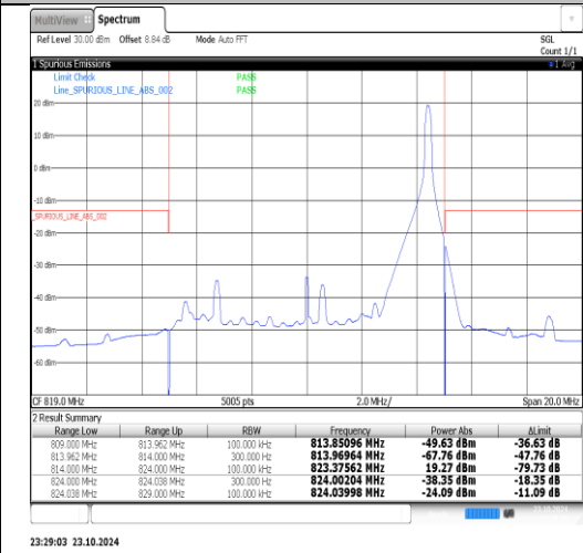
Band26(824-849)-1.4MHz-QPSK-26797-6RB#0-PASS
