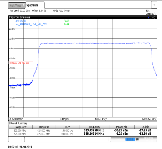
Band26(824-849)-5MHz-QPSK-27015-1RB#0-PASS
