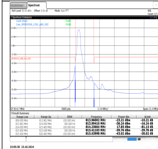
Band26(814-824)-1.4MHz-16QAM-26697-1RB#5-PASS
