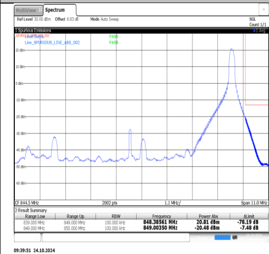
Band26(824-849)-15MHz-QPSK-26865-75RB#0-PASS
