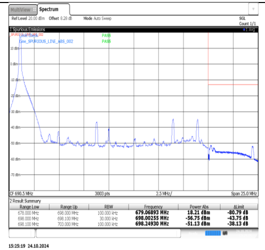
Band71-20MHz-16QAM-133372-1RB#99-PASS
