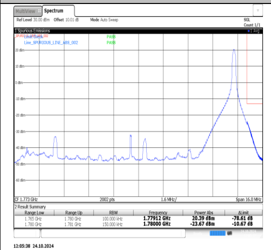
Band66-15MHz-16QAM-132047-75RB#0-PASS
