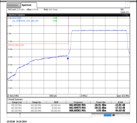
Band71-5MHz-QPSK-133447-1RB#0-PASS
