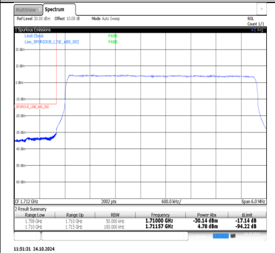
Band66-5MHz-16QAM-131997-25RB#0-PASS
