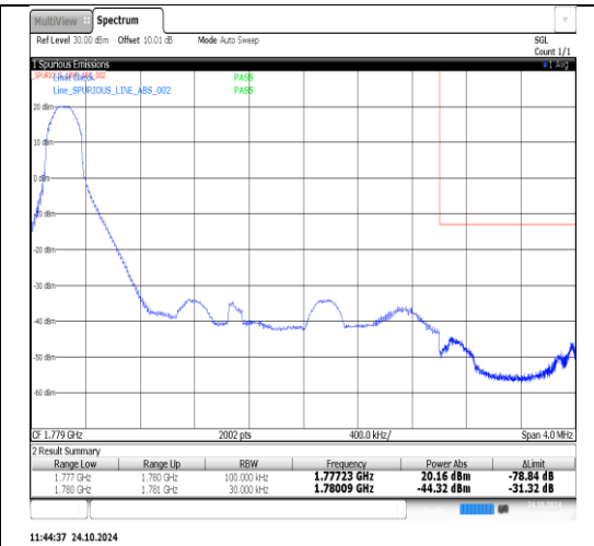
Band66-3MHz-QPSK-132657-1RB#14-PASS
