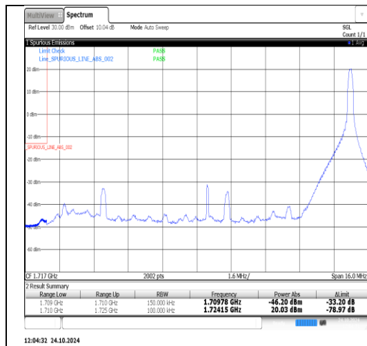
Band66-15MHz-QPSK-132597-75RB#0-PASS
