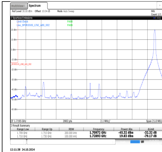
Band66-20MHz-QPSK-132572-100RB#0-PASS
