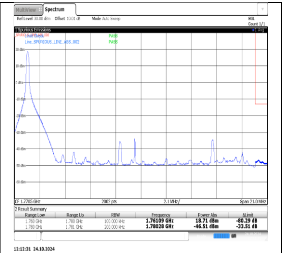
Band66-20MHz-16QAM-132572-1RB#99-PASS
