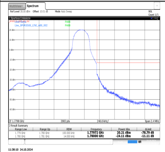
Band66-1.4MHz-16QAM-131979-6RB#0-PASS
