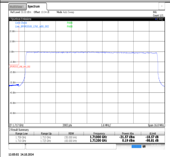
Band66-15MHz-16QAM-132597-1RB#0-PASS
