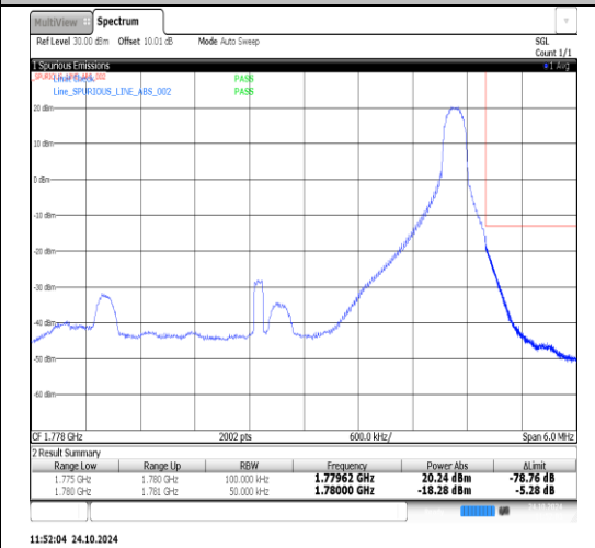
Band66-5MHz-QPSK-132647-1RB#24-PASS
