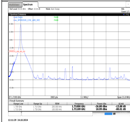
Band66-20MHz-16QAM-132072-1RB#99-PASS
