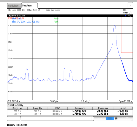
Band66-10MHz-16QAM-132022-50RB#0-PASS
