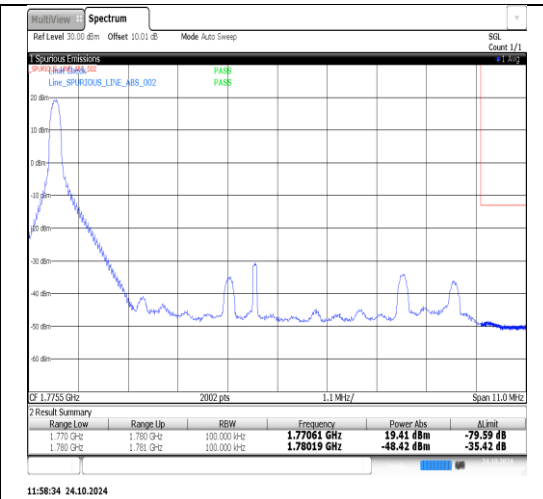
Band66-10MHz-16QAM-132622-1RB#49-PASS
