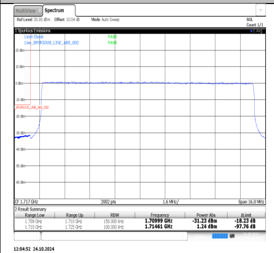
Band66-15MHz-QPSK-132597-1RB#0-PASS
