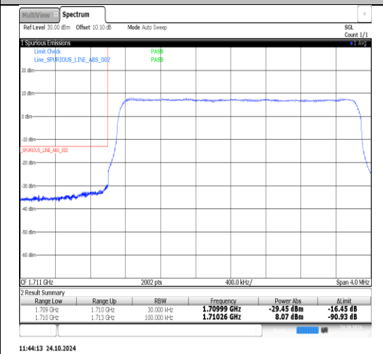
Band66-3MHz-QPSK-132657-1RB#0-PASS
