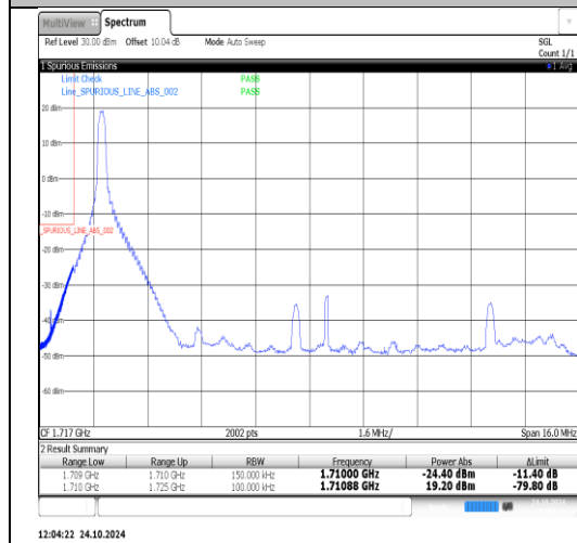
Band66-15MHz-16QAM-132047-1RB#74-PASS
