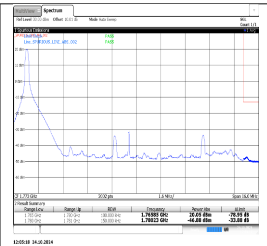
Band66-15MHz-QPSK-132597-1RB#74-PASS
