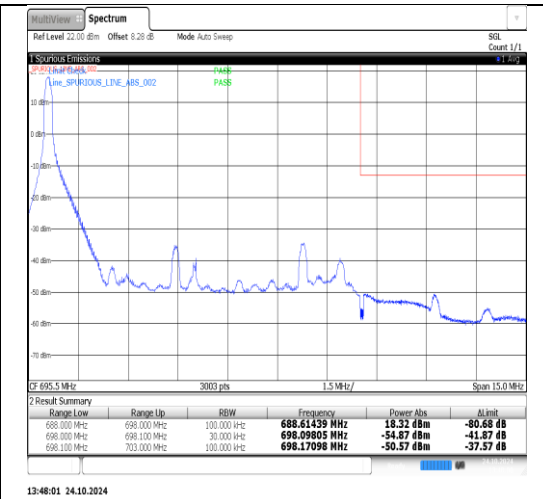
Band71-10MHz-16QAM-133422-1RB#49-PASS
