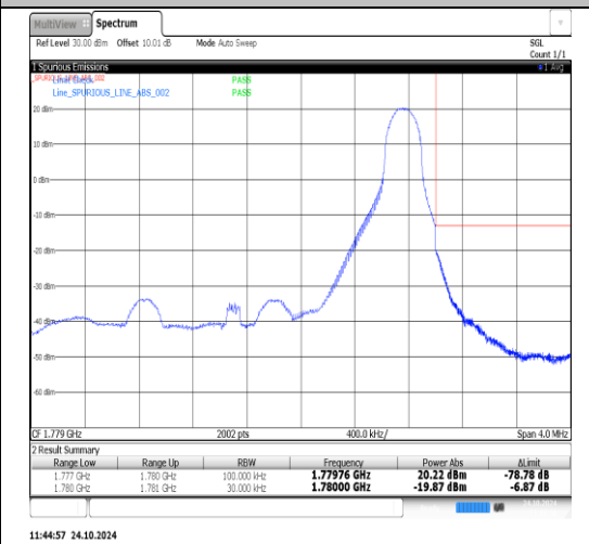
Band66-3MHz-16QAM-131987-15RB#0-PASS
