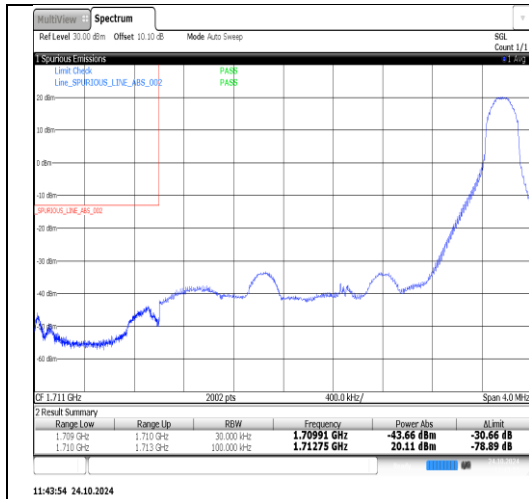
Band66-3MHz-QPSK-132657-15RB#0-PASS
