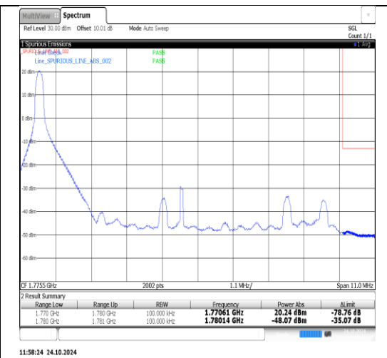
Band66-10MHz-QPSK-132622-1RB#49-PASS
