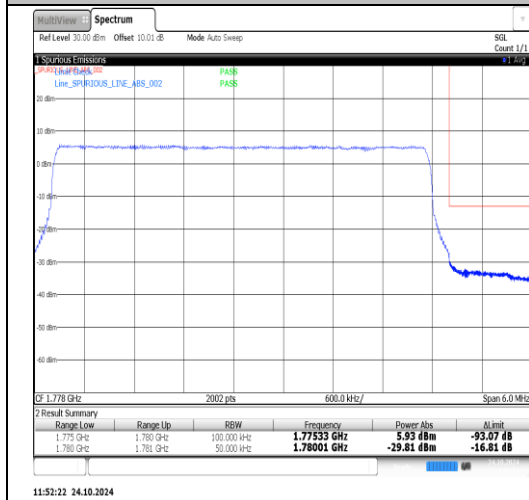
Band66-5MHz-QPSK-132647-25RB#0-PASS
