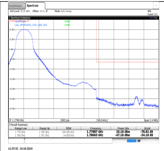
Band66-1.4MHz-QPSK-132665-1RB#5-PASS
