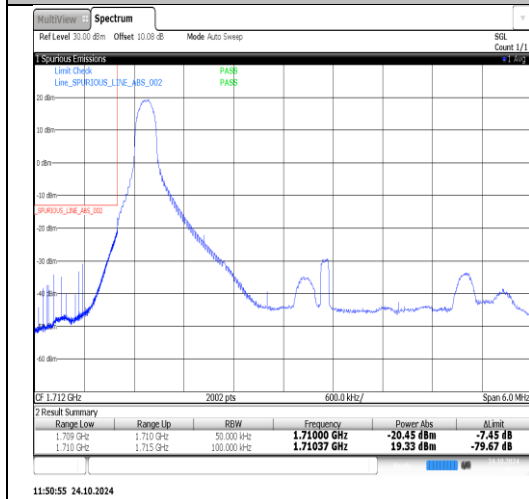
Band66-5MHz-16QAM-131997-1RB#0-PASS
