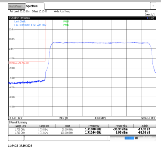
Band66-3MHz-16QAM-132657-1RB#0-PASS
