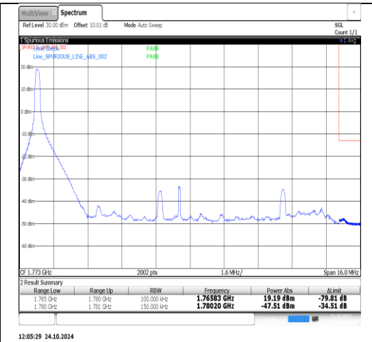
Band66-15MHz-16QAM-132597-1RB#74-PASS
