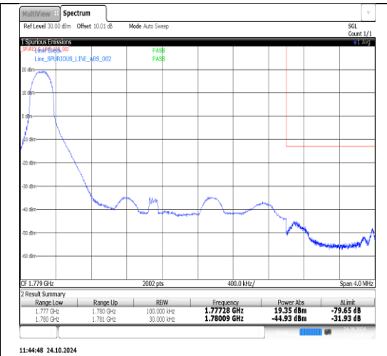
Band66-3MHz-16QAM-132657-1RB#14-PASS
