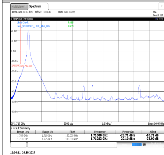
Band66-15MHz-QPSK-132047-1RB#74-PASS
