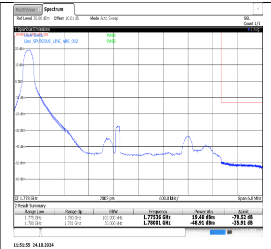
Band66-5MHz-16QAM-132647-1RB#24-PASS
