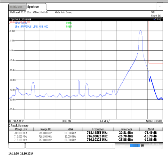
Band17-10MHz-16QAM-23780-50RB#0-PASS
