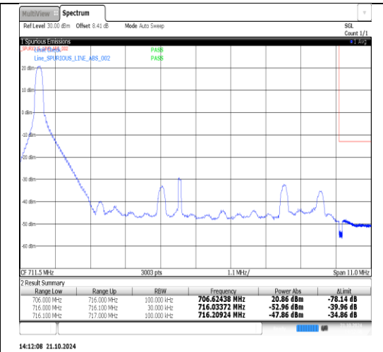
Band17-10MHz-QPSK-23800-1RB#49-PASS
