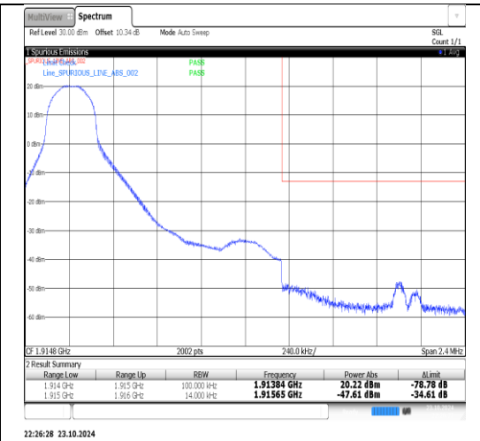
Band25-1.4MHz-QPSK-26683-1RB#5-PASS
