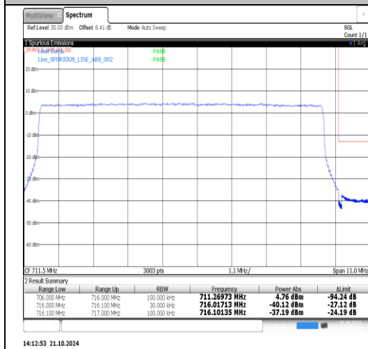
Band17-10MHz-16QAM-23780-1RB#0-PASS
