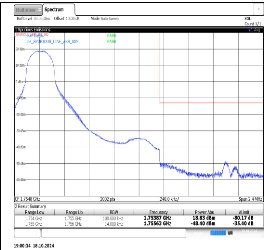
Band4-1.4MHz-16QAM-20393-1RB#5-PASS
