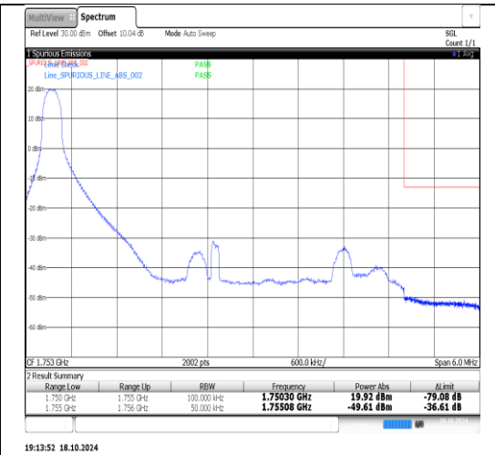
Band4-5MHz-QPSK-20375-1RB#24-PASS
