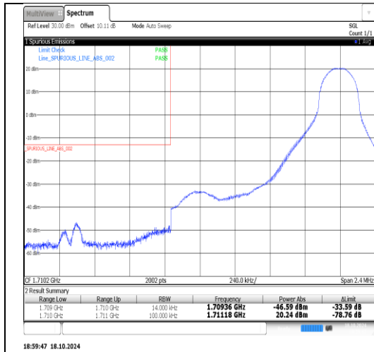
Band4-1.4MHz-QPSK-20393-6RB#0-PASS
