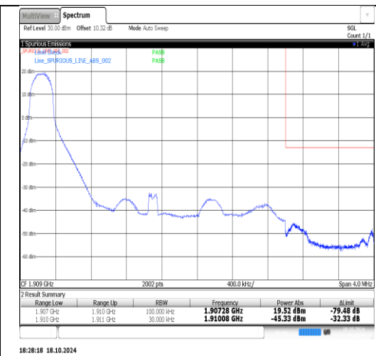
Band2-3MHz-16QAM-19185-1RB#14-PASS
