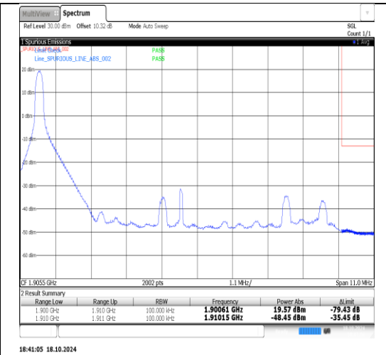
Band2-10MHz-16QAM-19150-1RB#49-PASS
