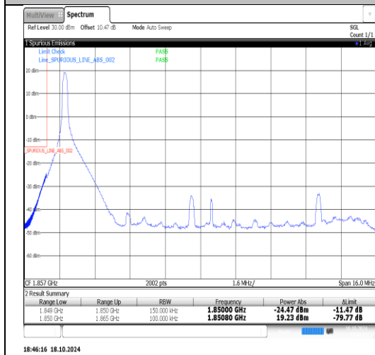
Band2-15MHz-QPSK-18675-1RB#74-PASS
