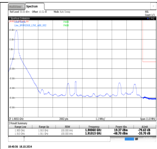
Band2-10MHz-QPSK-19150-1RB#49-PASS
