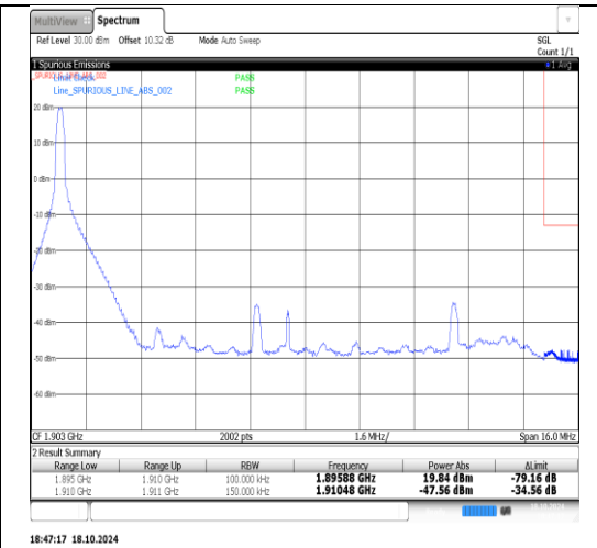
Band2-15MHz-QPSK-19125-1RB#74-PASS
