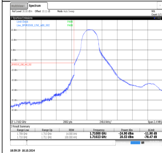
Band4-1.4MHz-QPSK-19957-1RB#5-PASS
