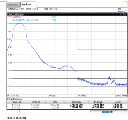
Band4-1.4MHz-QPSK-20393-1RB#5-PASS
