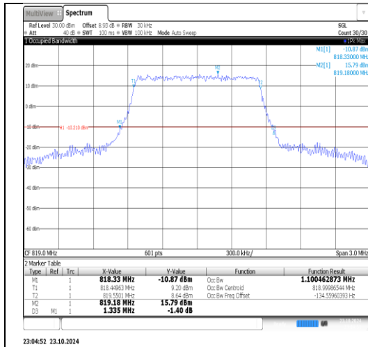
Band26(814-824)-3MHz-QPSK-26740-15RB#0-PASS
