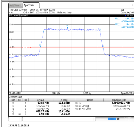
Band71-10MHz-QPSK-133297-50RB#0-PASS
