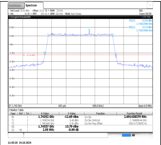
Band66-5MHz-16QAM-132322-25RB#0-PASS
