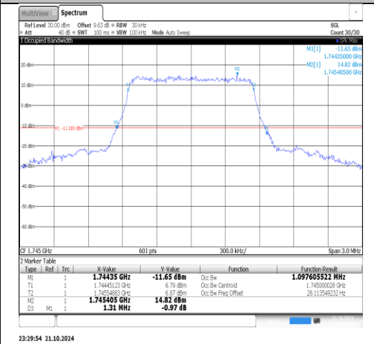
Band66-3MHz-16QAM-132322-15RB#0-PASS
