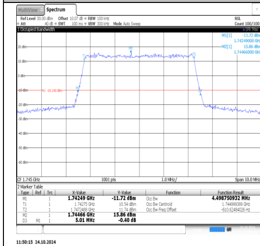
Band66-10MHz-QPSK-132322-50RB#0-PASS
