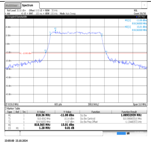
Band26(814-824)-3MHz-16QAM-26740-15RB#0-PASS
