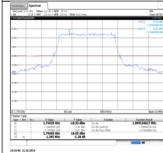
Band66-3MHz-QPSK-132322-15RB#0-PASS
