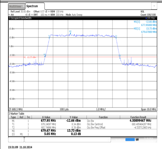
Band71-10MHz-16QAM-133297-50RB#0-PASS
