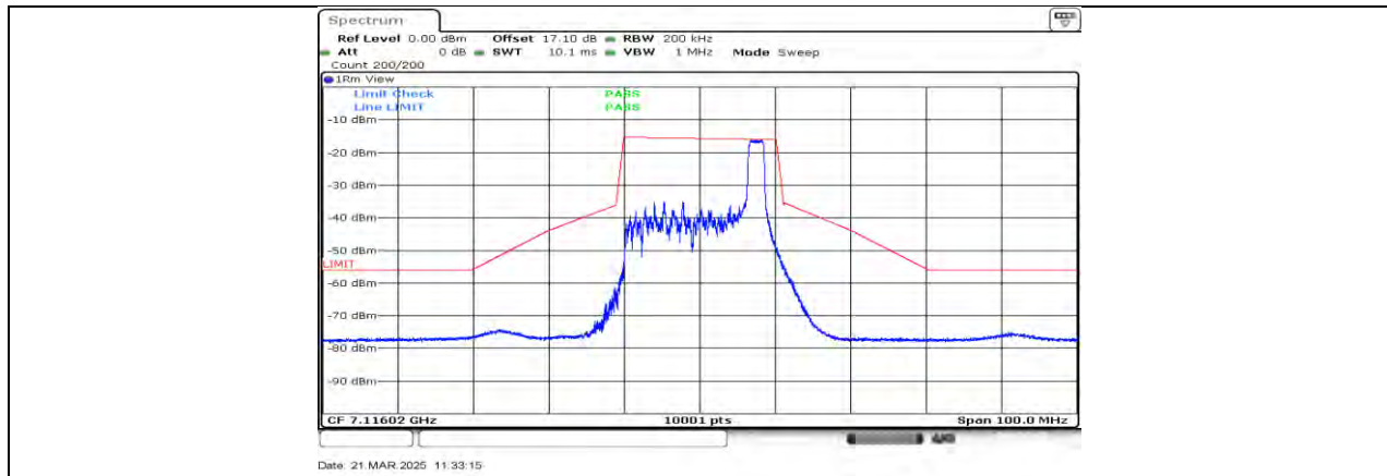
11AX20MIMO Ant1_7115_26Tone_RU8
