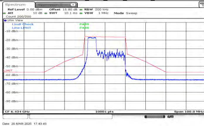
11AX20MIMO Ant1_6435_52Tone_RU37
