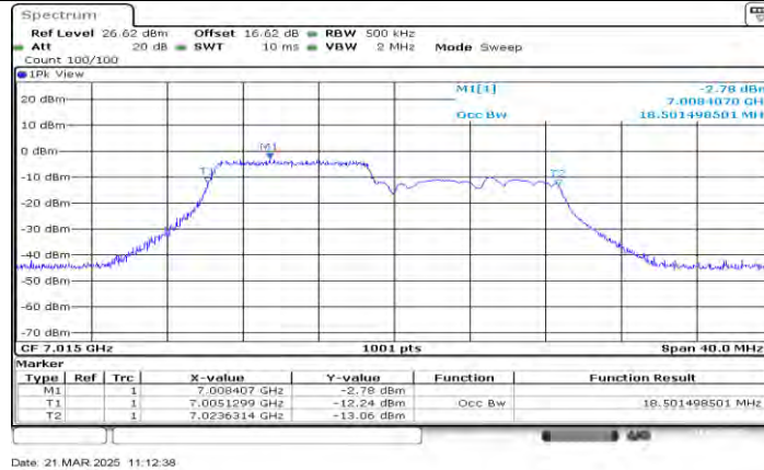
11AX20MIMO Ant1_7015_106Tone_RU53
