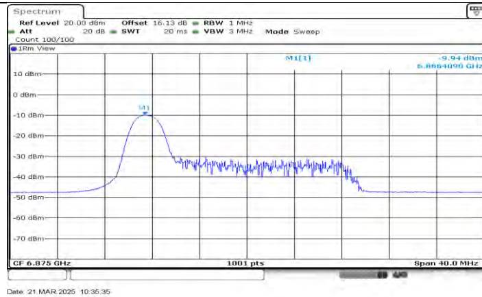
11AX20MIMO Ant2_6875_26Tone_RU0
