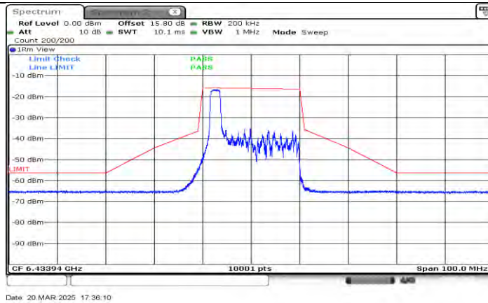
11AX20MIMO Ant1_6435_26Tone_RU0
