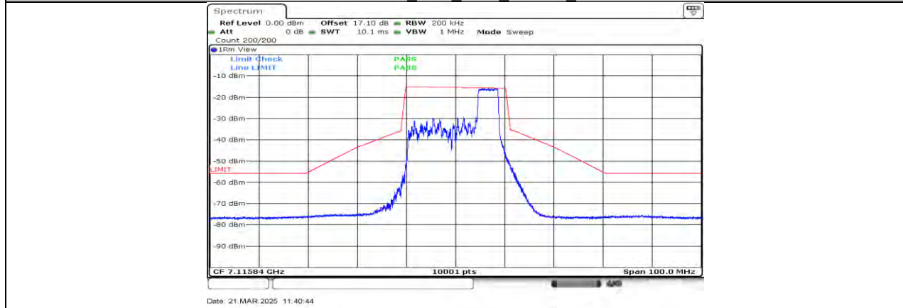
11AX20MIMO Ant1_7115_52Tone_RU40
