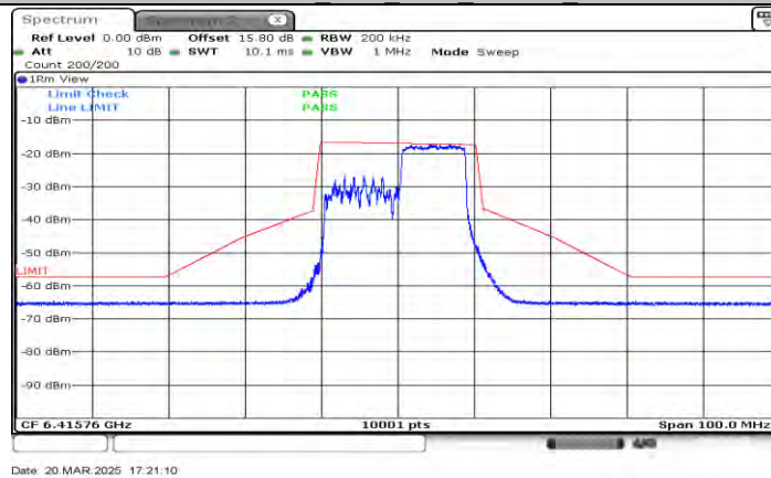
11AX20MIMO Ant1_6415_106Tone_RU54
