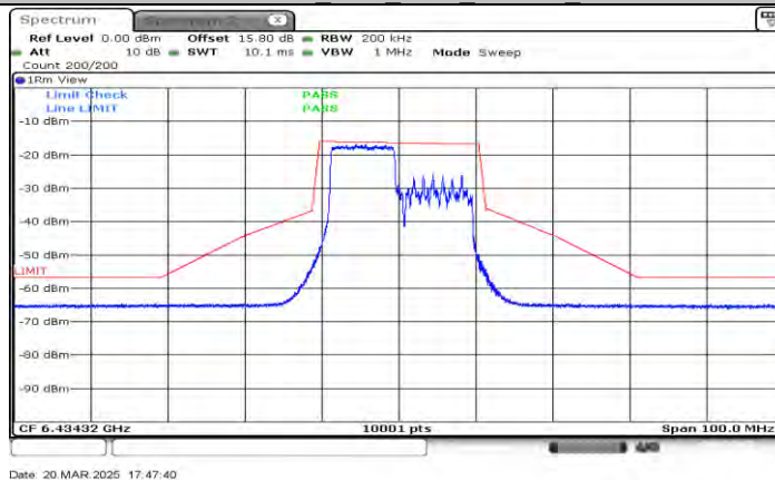
11AX20MIMO Ant1_6435_106Tone_RU53
