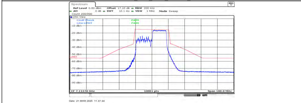
11AX20MIMO Ant1_7115_106Tone_RU54
