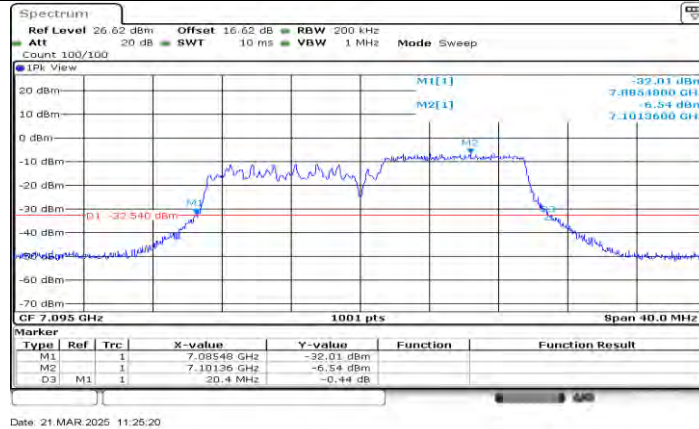
11AX20MIMO Ant1_7095_106Tone_RU54
