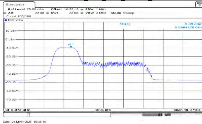
11AX20MIMO Ant2_6875_52Tone_RU37
