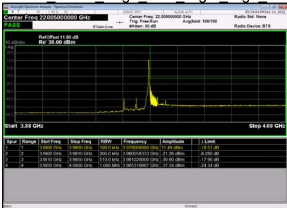
N77(20M)_DFT-s- OFDM BPSK Edge 1RB Right High CH
