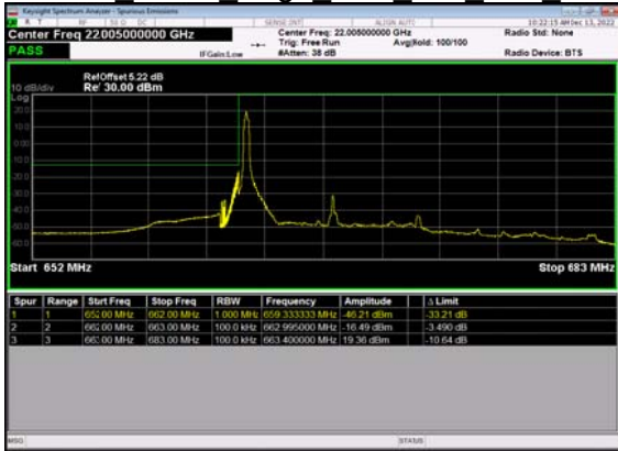
N71(10M)_DFT-s- OFDM BPSK Edge 1RB Left Low CH
