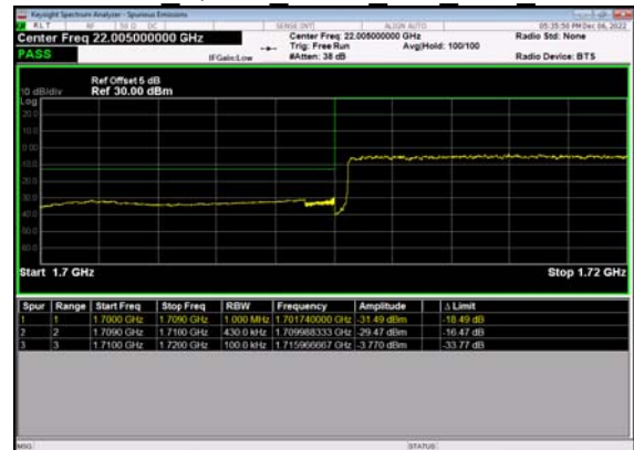
N66(40M)_DFT-s- OFDM QPSK Outer Full Low CH
