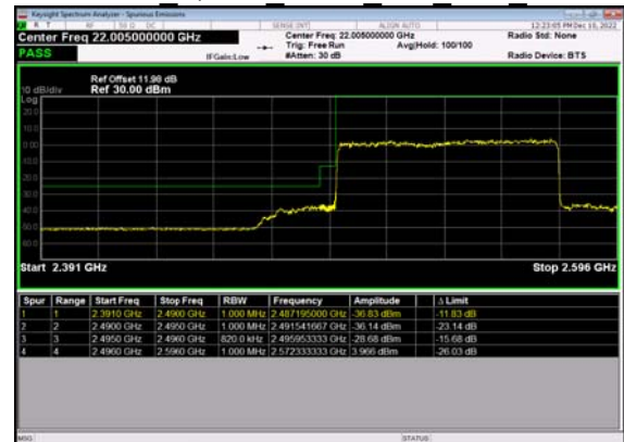
N41(80M)_DFT-s- OFDM QPSK Outer Full Low CH
