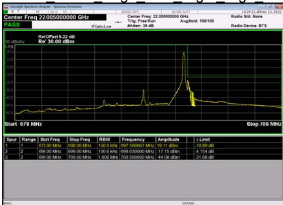
N71(10M)_DFT-s- OFDM BPSK Edge 1RB Right High CH
