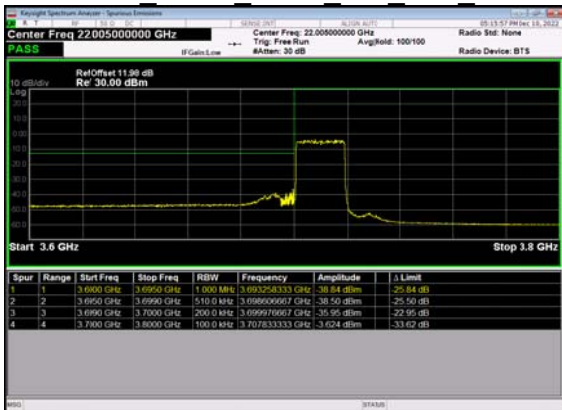
N77(20M)_DFT-s- OFDM BPSK Outer Full Low CH
