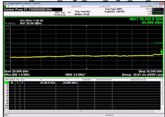
N77(90M)_DFT-s- OFDM_QPSK_Edge_1RB_Right_Mid_CH
