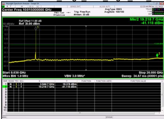
N77(90M)_DFT-s-OFDM_QPSK_Edge_1RB_Right_Mid_CH
