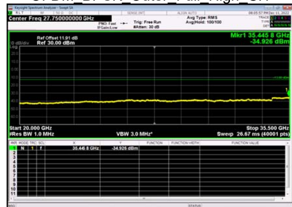
N77(15M)_DFT-s- OFDM BPSK Outer Full High CH
