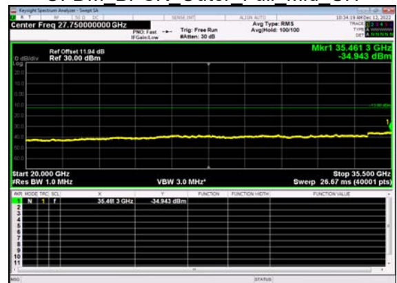
N77(20M)_DFT-s- OFDM BPSK Outer Full Mid CH
