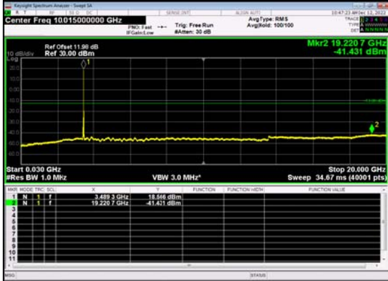
N77(40M)_DFT-s- OFDM BPSK Edge 1RB Right Low CH
