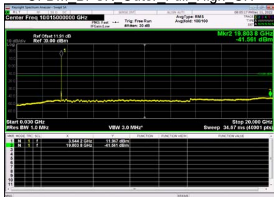
N77(15M)_DFT-s- OFDM BPSK Outer Full High CH
