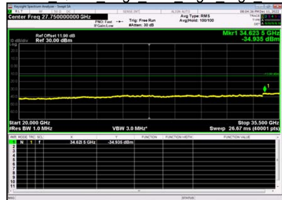
N77(15M)_DFT-s- OFDM QPSK Edge 1RB Right High CH
