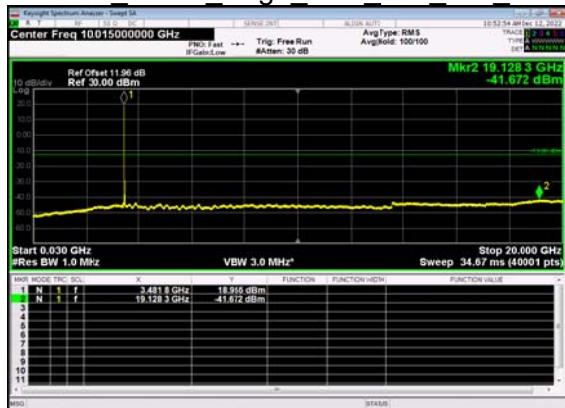
N77(40M)_DFT-s- OFDM BPSK Edge 1RB Left Mid CH
