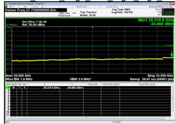
N77(15M)_DFT-s- OFDM BPSK Edge 1RB Right High CH
