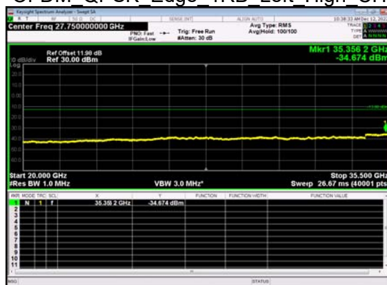
N77(20M)_DFT-s- OFDM QPSK Edge 1RB Left High CH
