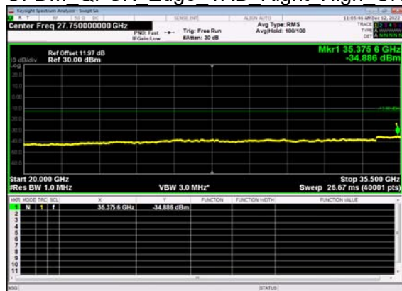
N77(40M)_DFT-s- OFDM QPSK Edge 1RB Right High CH
