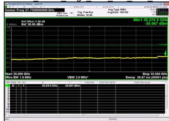
N77(40M)_DFT-s- OFDM BPSK Edge 1RB Left Low CH
