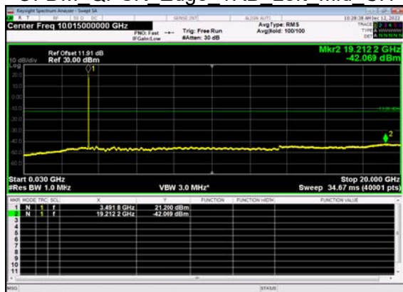
N77(20M)_DFT-s- OFDM QPSK Edge 1RB Left Mid CH
