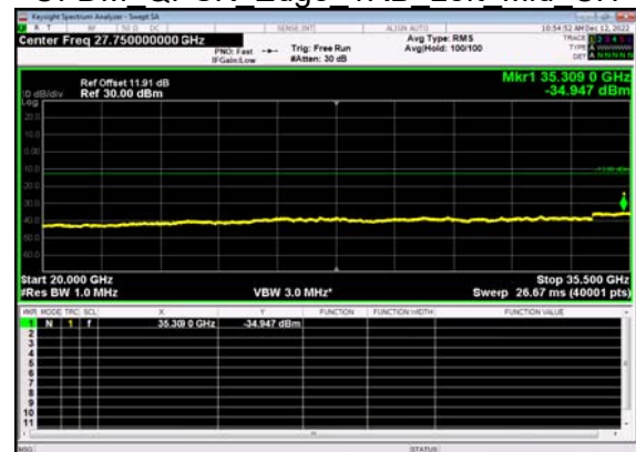
N77(40M)_DFT-s- OFDM QPSK Edge 1RB Left Mid CH
