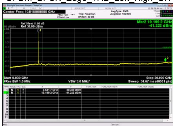
N77(20M)_DFT-s- OFDM BPSK Edge 1RB Left High CH
