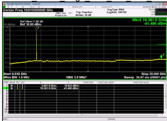
N77(40M)_DFT-s- OFDM BPSK Edge 1RB Left Low CH
