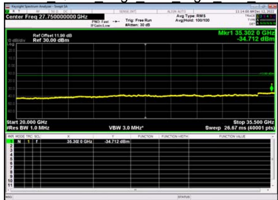
N77(50M)_DFT-s- OFDM QPSK Edge 1RB Right Low CH
