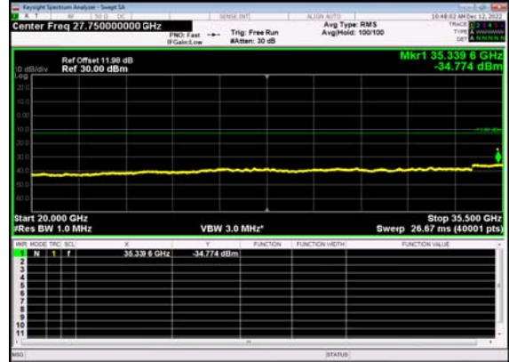
N77(40M)_DFT-s- OFDM BPSK Edge 1RB Right Low CH
