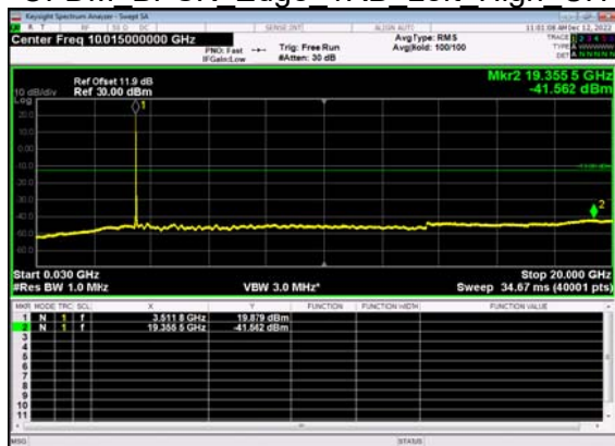
N77(40M)_DFT-s- OFDM BPSK Edge 1RB Left High CH
