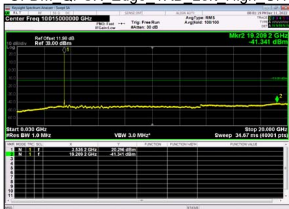
N77(15M)_DFT-s- OFDM QPSK Edge 1RB Left High CH
