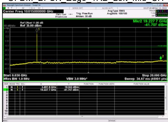
N77(20M)_DFT-s- OFDM BPSK Edge 1RB Left Mid CH
