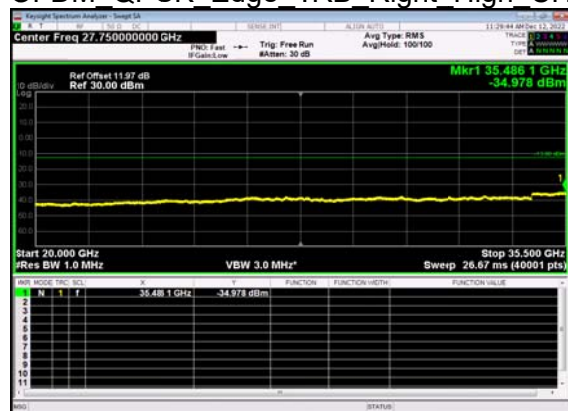
N77(50M)_DFT-s-OFDM QPSK Edge 1RB Right High CH
